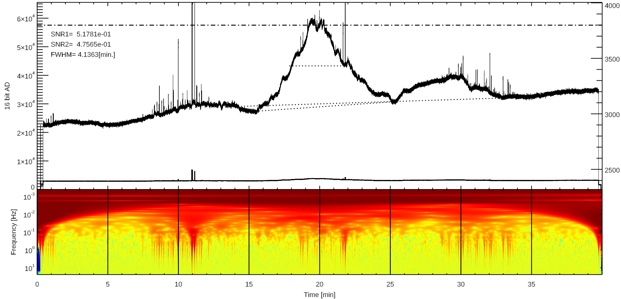
C 3C348 (/home4/archive/swift/dat/2023/07/T20230706212553.dat)
