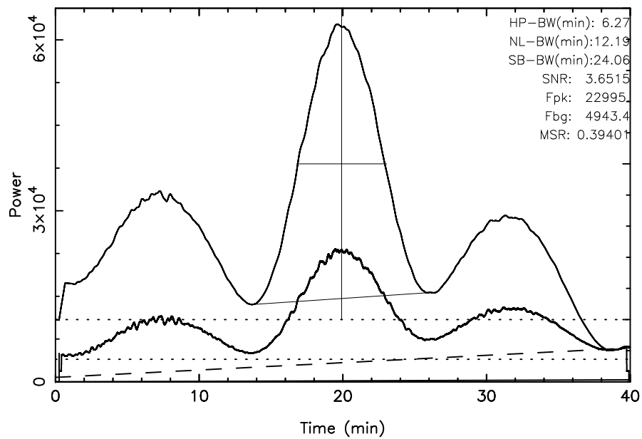
TOYOKAWA 3C405 2023/07/07(188)00:33:19-01:13:19JST
