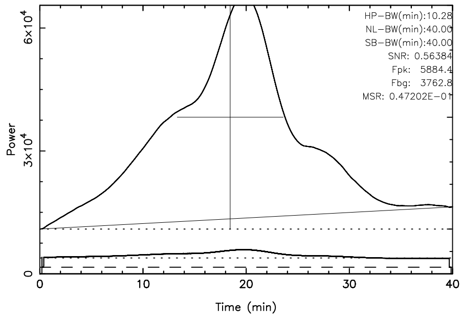
TOYOKAWA 3C392 2023/07/10(191)23:14:46-23:54:46JST
