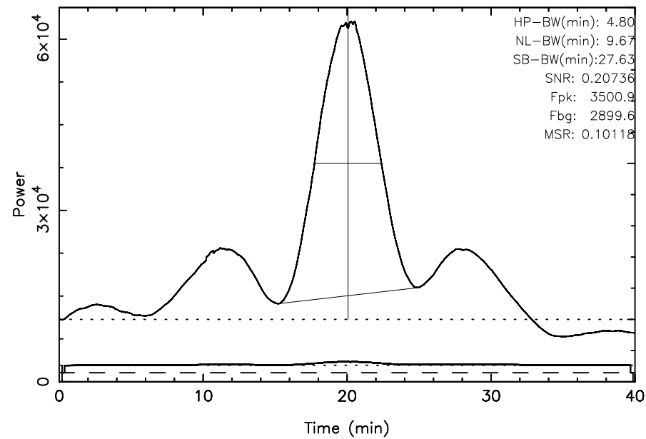
TOYOKAWA 3C348 2023/07/10(191)21:10:07-21:50:07JST
