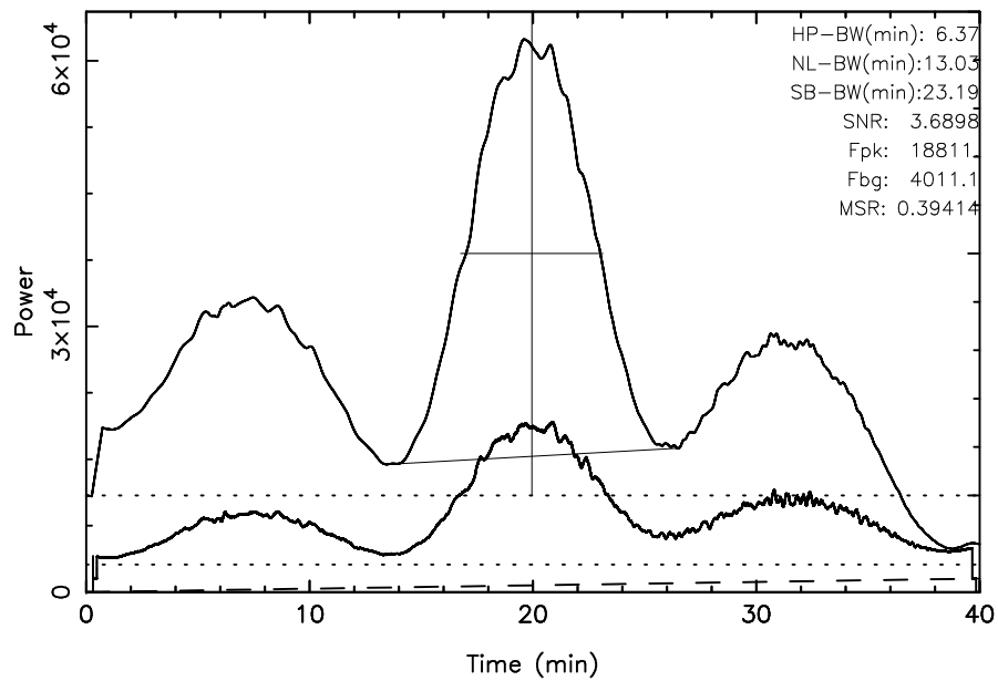
TOYOKAWA 3C405 2023/07/10(191)00:21:31-01:01:31JST
