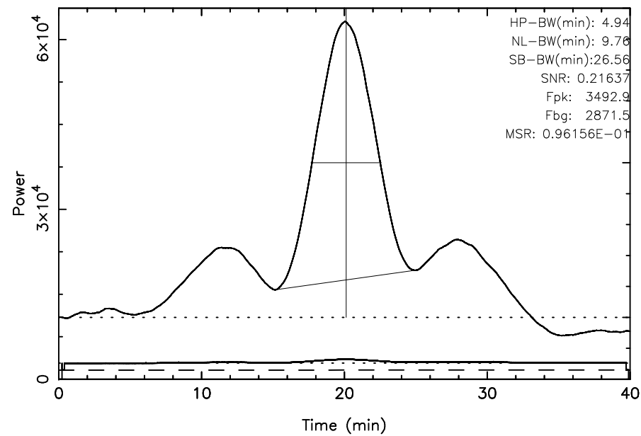
TOYOKAWA 3C348 2023/07/19(200)20:34:44-21:14:44JST
