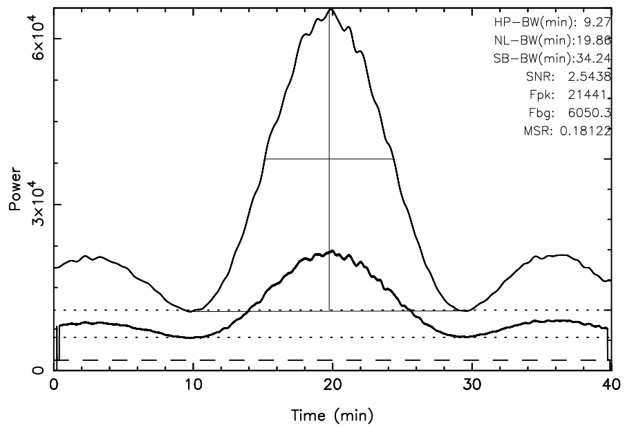
TOYOKAWA 3C461 2023/07/19(200)03:09:44-03:49:44JST
