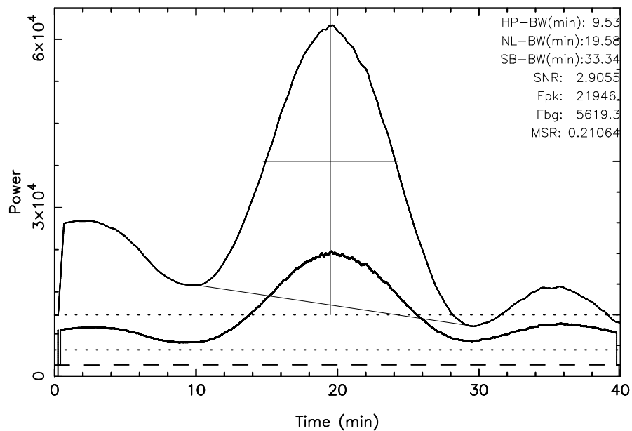
TOYOKAWA 3C461 2023/07/27(208)02:38:16-03:18:16JST
