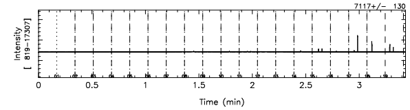
TOYOKAWA 3C286 2023/07/13(194)17:57:03-18:00:29JST
