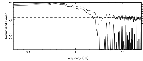
TOYOKAWA 3C286 2023/07/13(194)17:57:03-18:00:29JST
