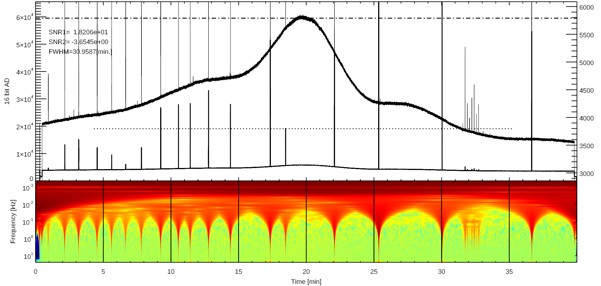
C 3C392 (/home4/archive/swift/dat/2023/08/T20230806212838.dat)
