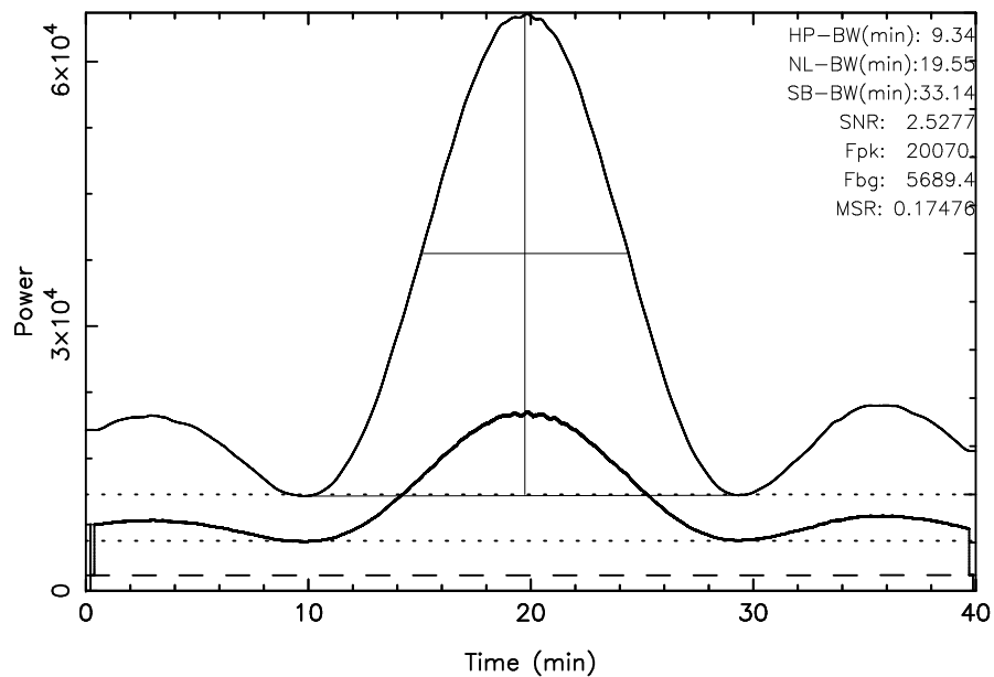
TOYOKAWA 3C461 2023/08/02(214)02:14:41-02:54:41JST
