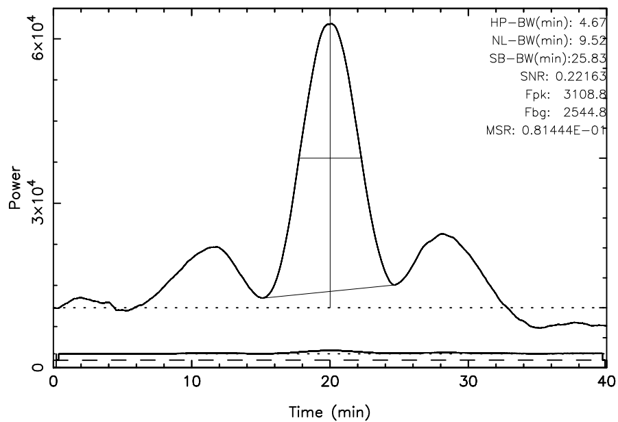
TOYOKAWA 3C348 2023/08/08(220)19:16:06-19:56:06JST
