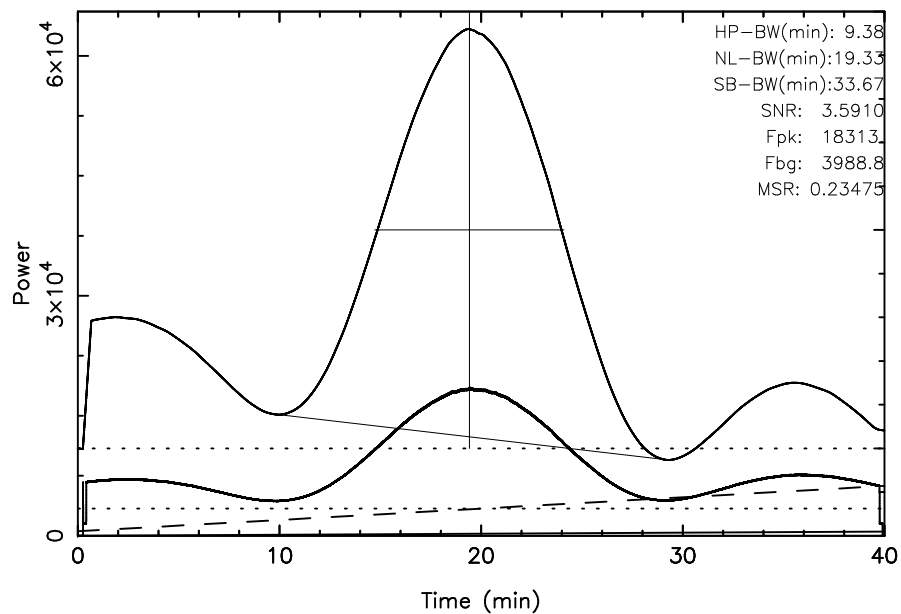
TOYOKAWA 3C461 2023/08/18(230)01:11:47-01:51:47JST
