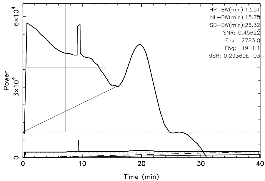
TOYOKAWA 3C348 2023/08/18(230)18:36:47-19:16:47JST
