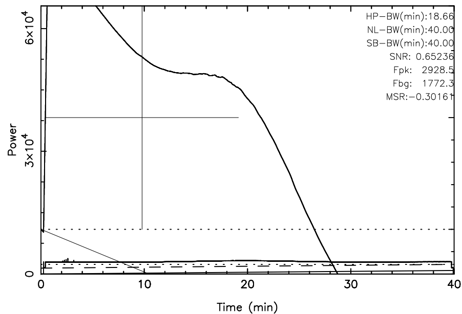
TOYOKAWA 3C10 2023/08/18(230)02:13:54-02:53:54JST
