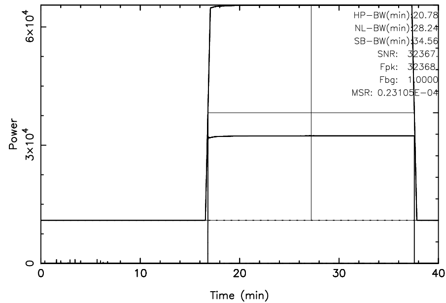
TOYOKAWA 3C392 2023/08/26(238)20:09:58-20:49:58JST
