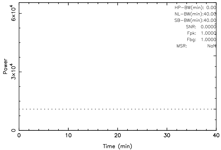
TOYOKAWA 3C461 2023/08/26(238)00:40:19-01:20:19JST
