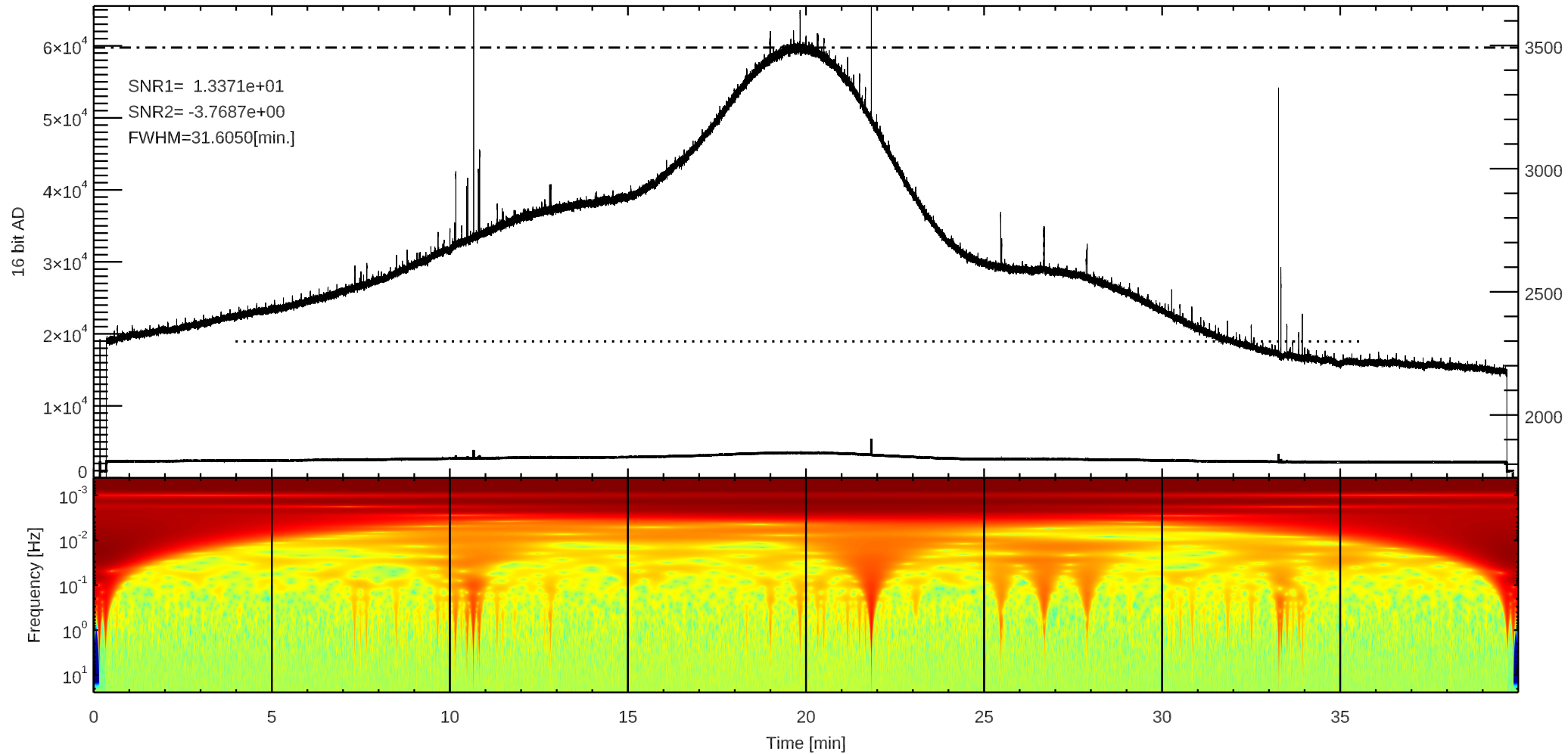
C 3C392 (/home4/archive/swift/dat/2023/09/T20230915185123.dat)
