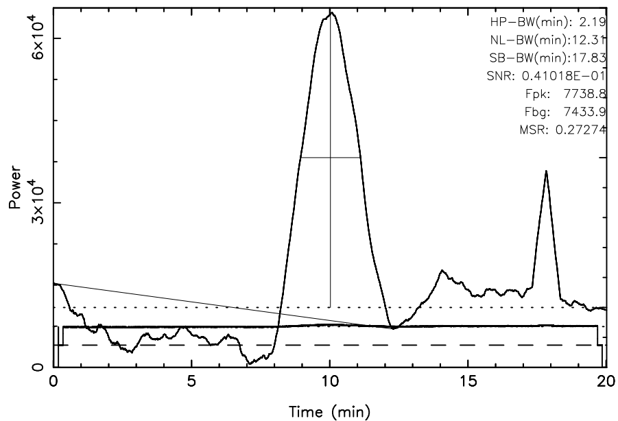
FUJI 3C123 2023/09/25(268)04:05:37-04:25:38JST
