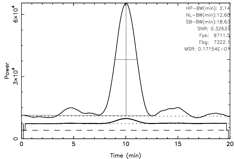
FUJI 3C144 2023/09/25(268)05:02:51-05:22:51JST
