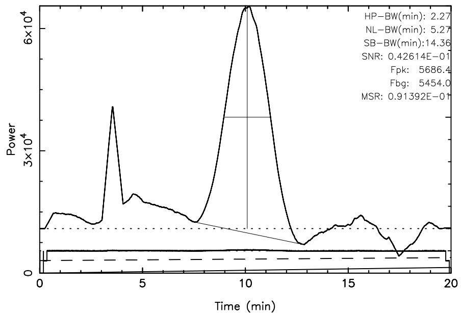
FUJI 3C123 2023/09/29(272)03:49:55-04:09:55JST
