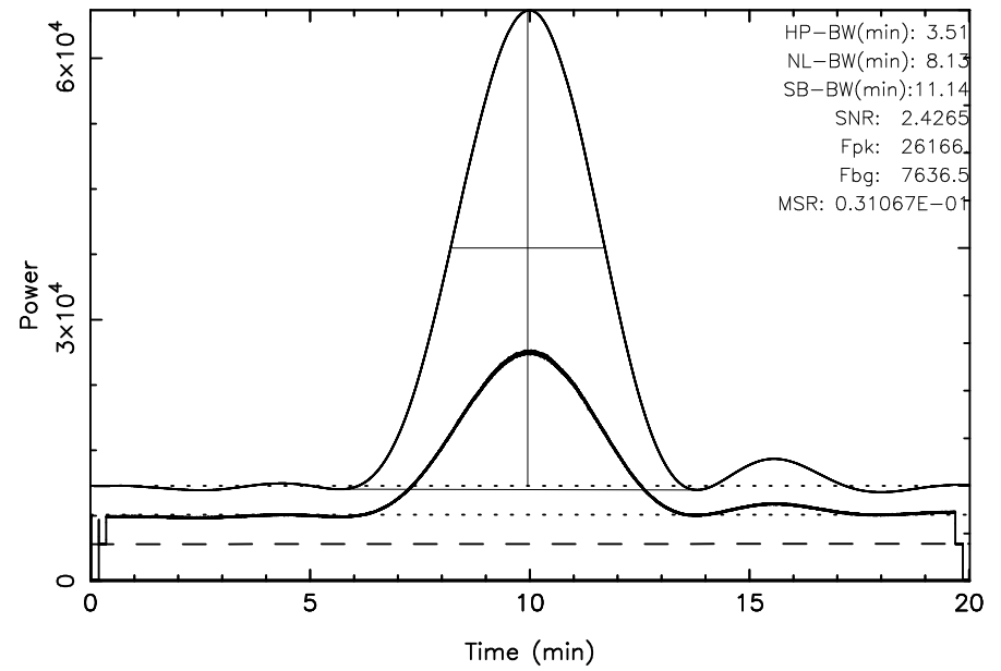
KISO 3C405 2023/09/29(272)19:09:06-19:29:07JST
