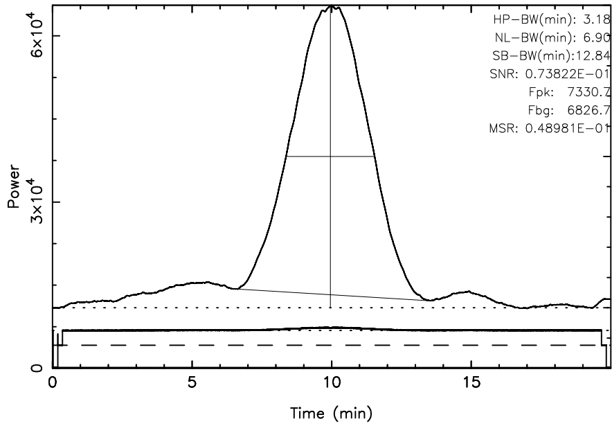
KISO 3C123 2023/09/29(272)03:49:55-04:09:55JST
