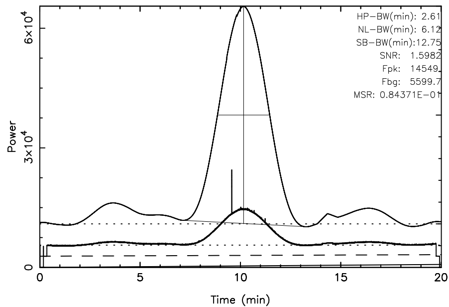
FUJI 3C405 2023/09/29(272)19:09:06-19:29:07JST
