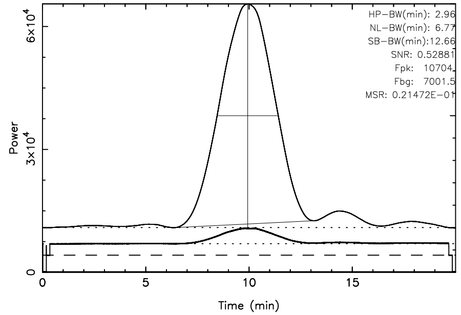
KISO 3C144 2023/09/29(272)04:47:07-05:07:07JST
