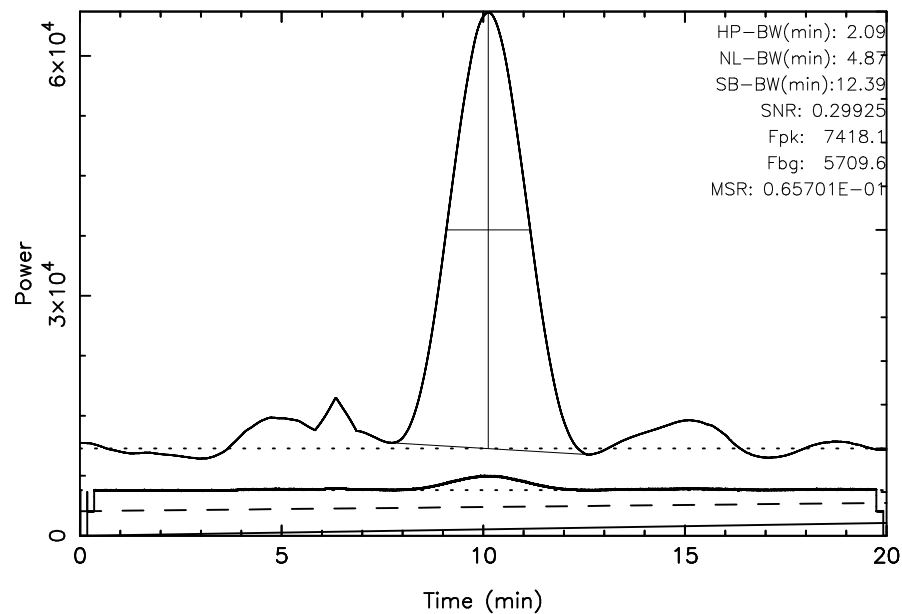
FUJI 3C144 2023/09/29(272)04:47:07-05:07:07JST
