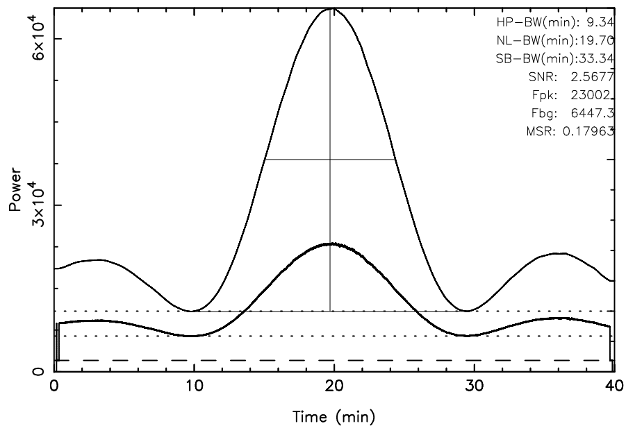
TOYOKAWA 3C461 2023/09/02(245)00:12:48-00:52:48JST
