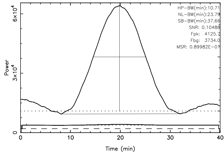
TOYOKAWA 3C10 2023/09/02(245)01:14:56-01:54:56JST
