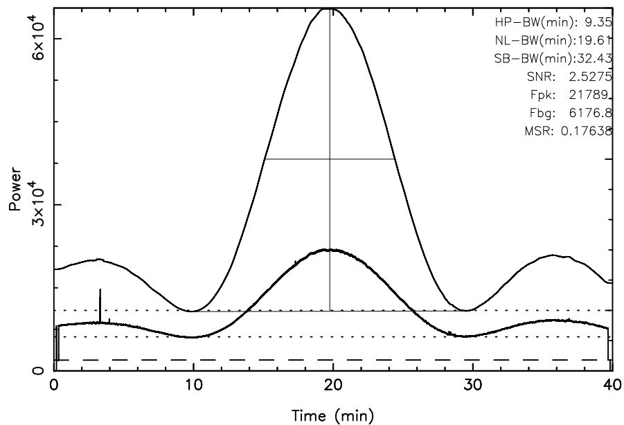
TOYOKAWA 3C461 2023/09/03(246)00:08:52-00:48:52JST
