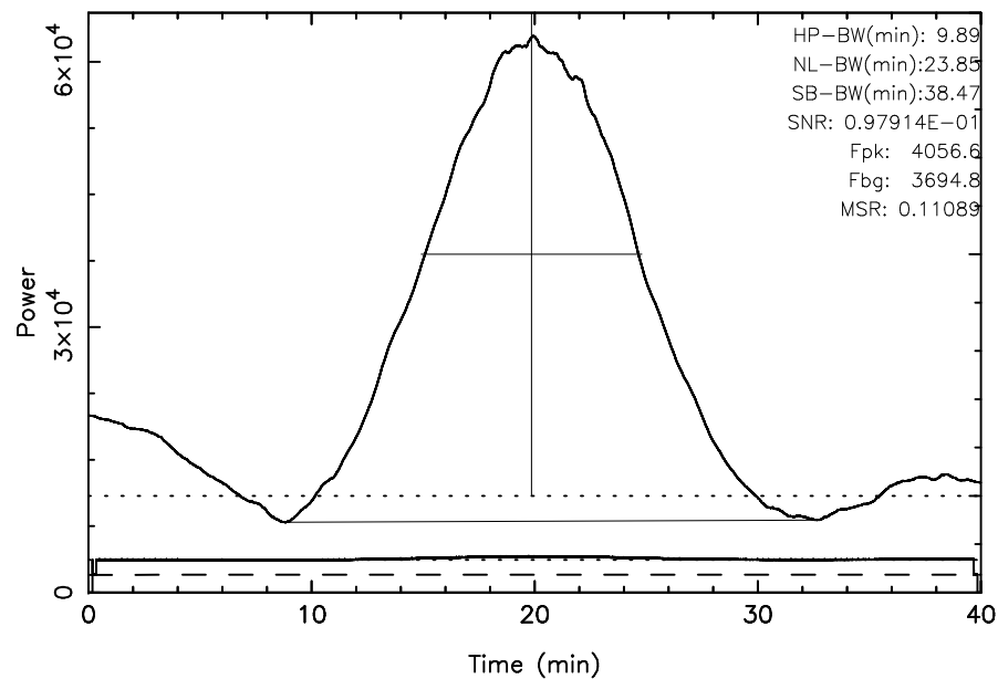
TOYOKAWA 3C10 2023/09/03(246)01:11:00-01:51:00JST
