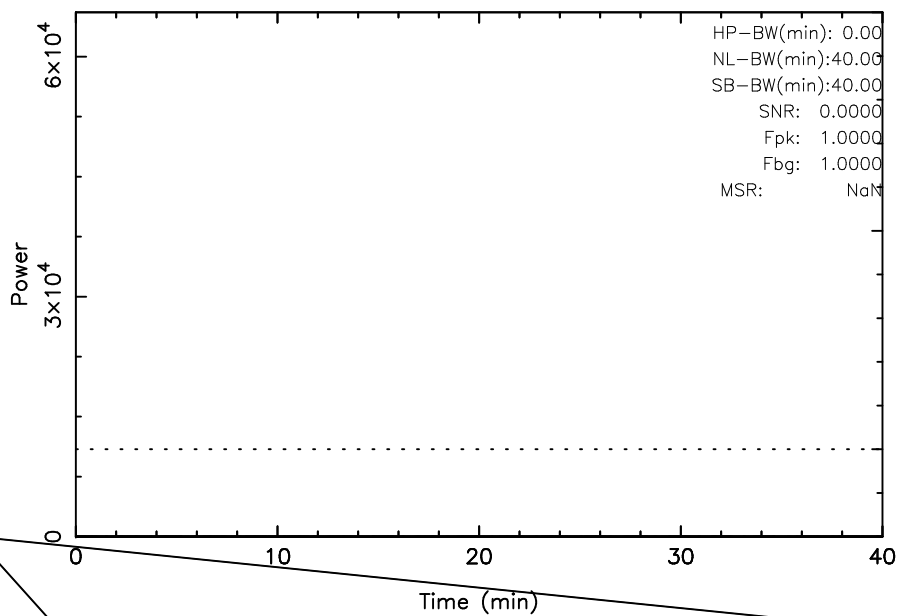
TOYOKAWA 3C392 2023/09/11(254)19:07:04-19:47:04JST
