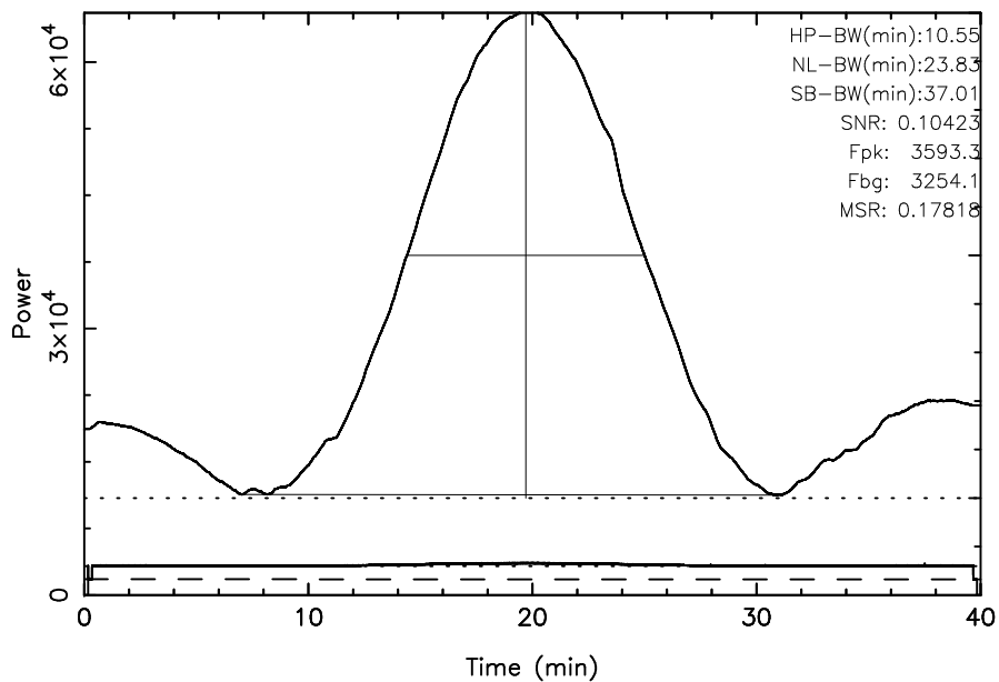
TOYOKAWA 3C10 2023/09/11(254)00:39:33-01:19:33JST
