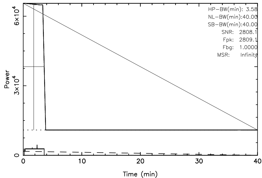
TOYOKAWA 3C123 2023/09/11(254)04:50:41-05:30:41JST
