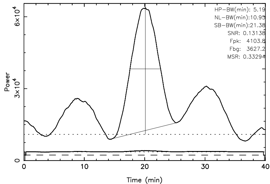
TOYOKAWA 3C123 2023/09/17(260)04:27:06-05:07:06JST
