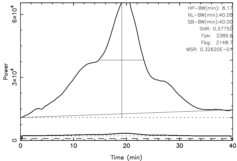
TOYOKAWA 3C392 2023/09/19(262)18:35:37-19:15:37JST
