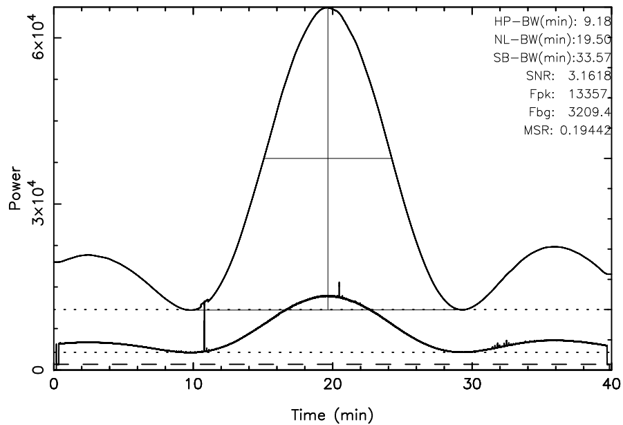
TOYOKAWA 3C461 2023/09/19(262)23:02:02-23:42:02JST
