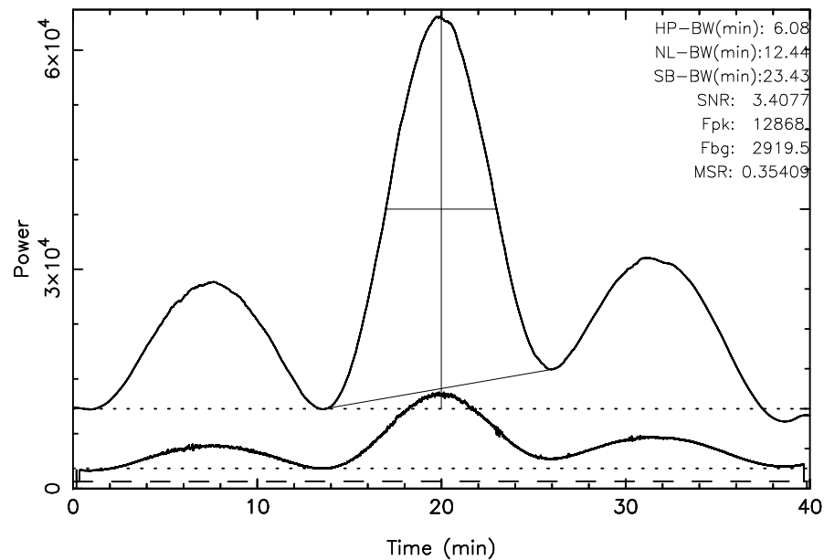
TOYOKAWA 3C405 2023/09/19(262)19:38:26-20:18:26JST
