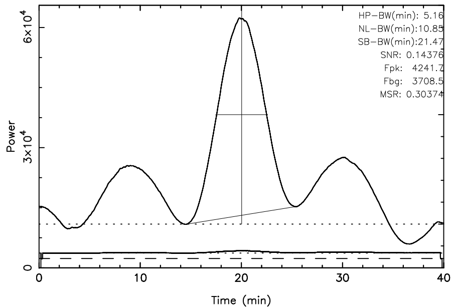
TOYOKAWA 3C123 2023/09/20(263)04:15:18-04:55:18JST
