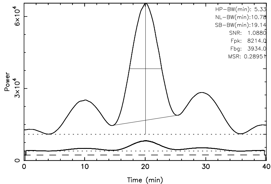
TOYOKAWA 3C144 2023/09/20(263)05:12:31-05:52:31JST
