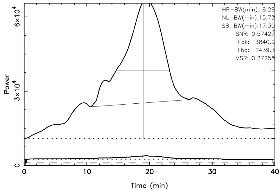
TOYOKAWA 3C392 2023/09/20(263)18:31:41-19:11:41JST
