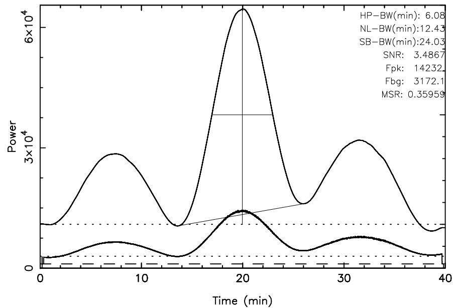
TOYOKAWA 3C405 2023/09/20(263)19:34:30-20:14:30JST
