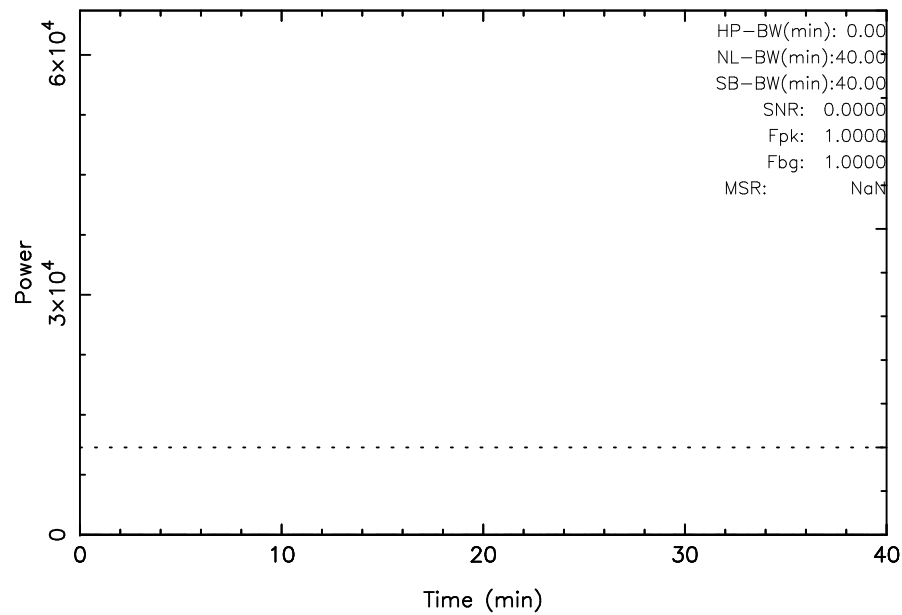
TOYOKAWA 3C144 2023/09/25(268)04:52:51-05:32:51JST
