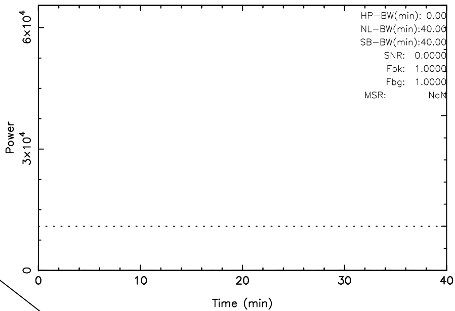
TOYOKAWA 3C123 2023/09/25(268)03:55:38-04:35:38JST
