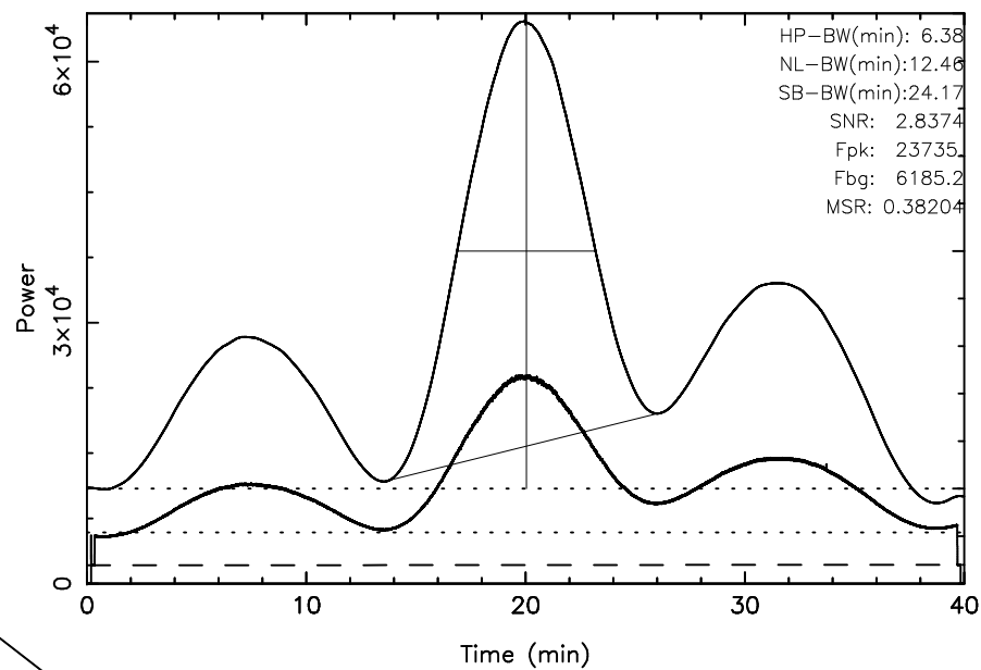
TOYOKAWA 3C405 2023/09/29(272)18:59:07-19:39:07JST
