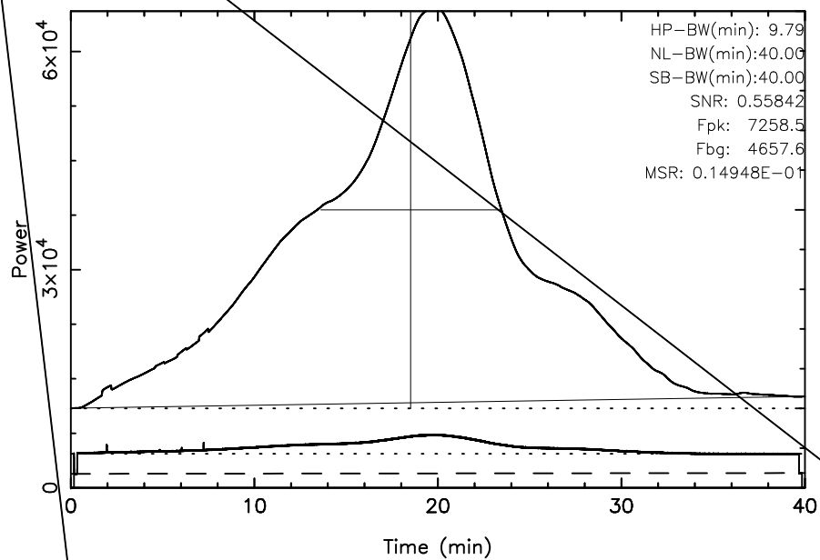
TOYOKAWA 3C392 2023/09/29(272)17:56:18-18:36:18JST
