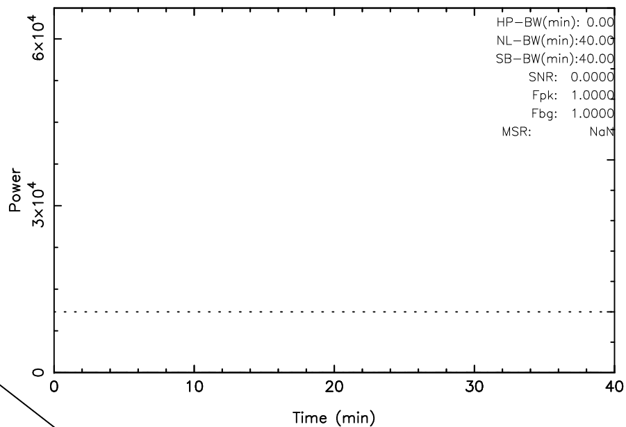
TOYOKAWA 3C123 2023/09/29(272)03:39:55-04:19:55JST
