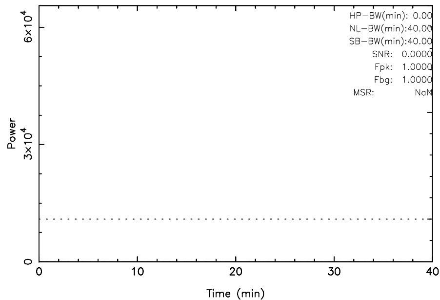
TOYOKAWA 3C144 2023/09/29(272)04:37:08-05:17:08JST
