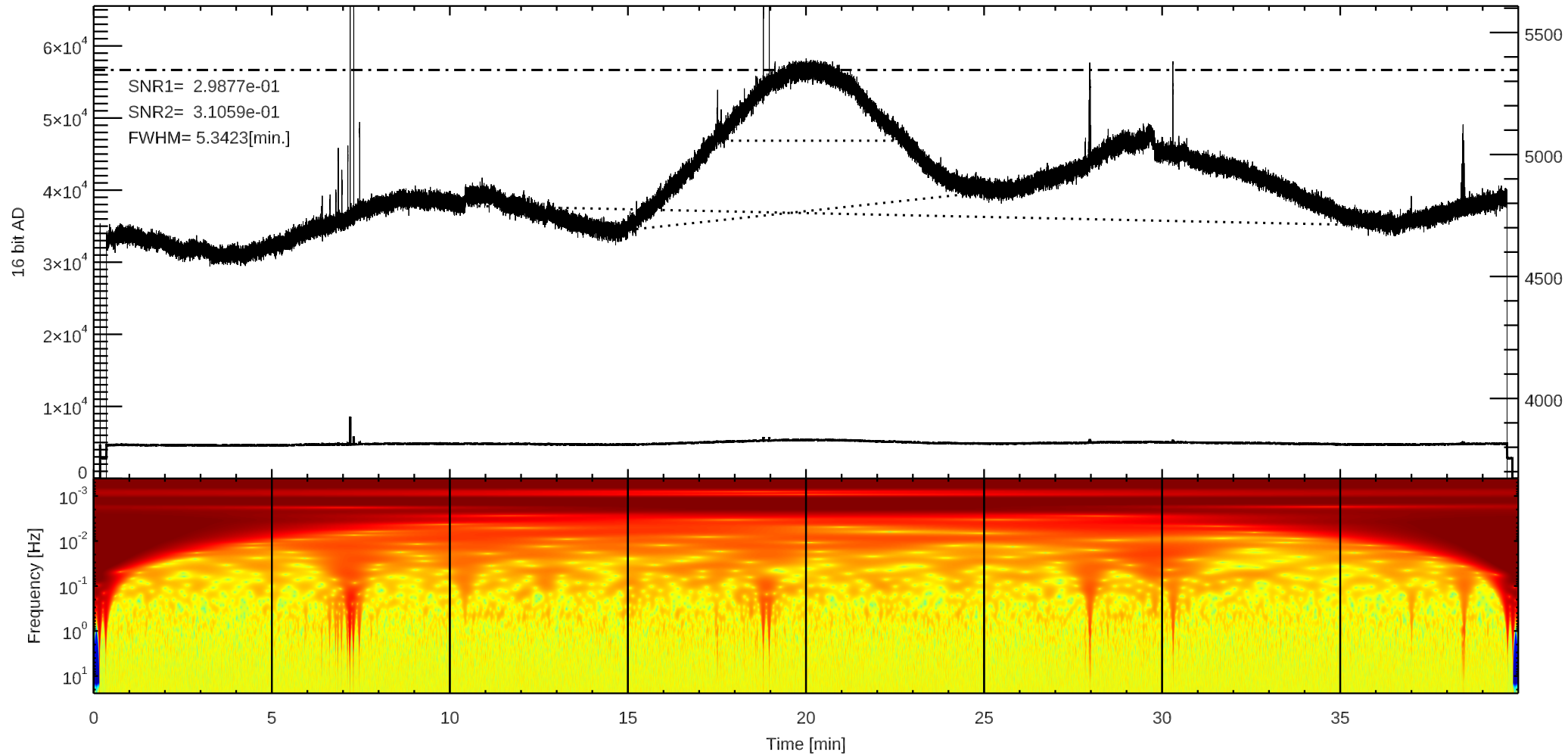
C 3C123 (/home4/archive/swift/dat/2023/10/T20231030013804.dat)
