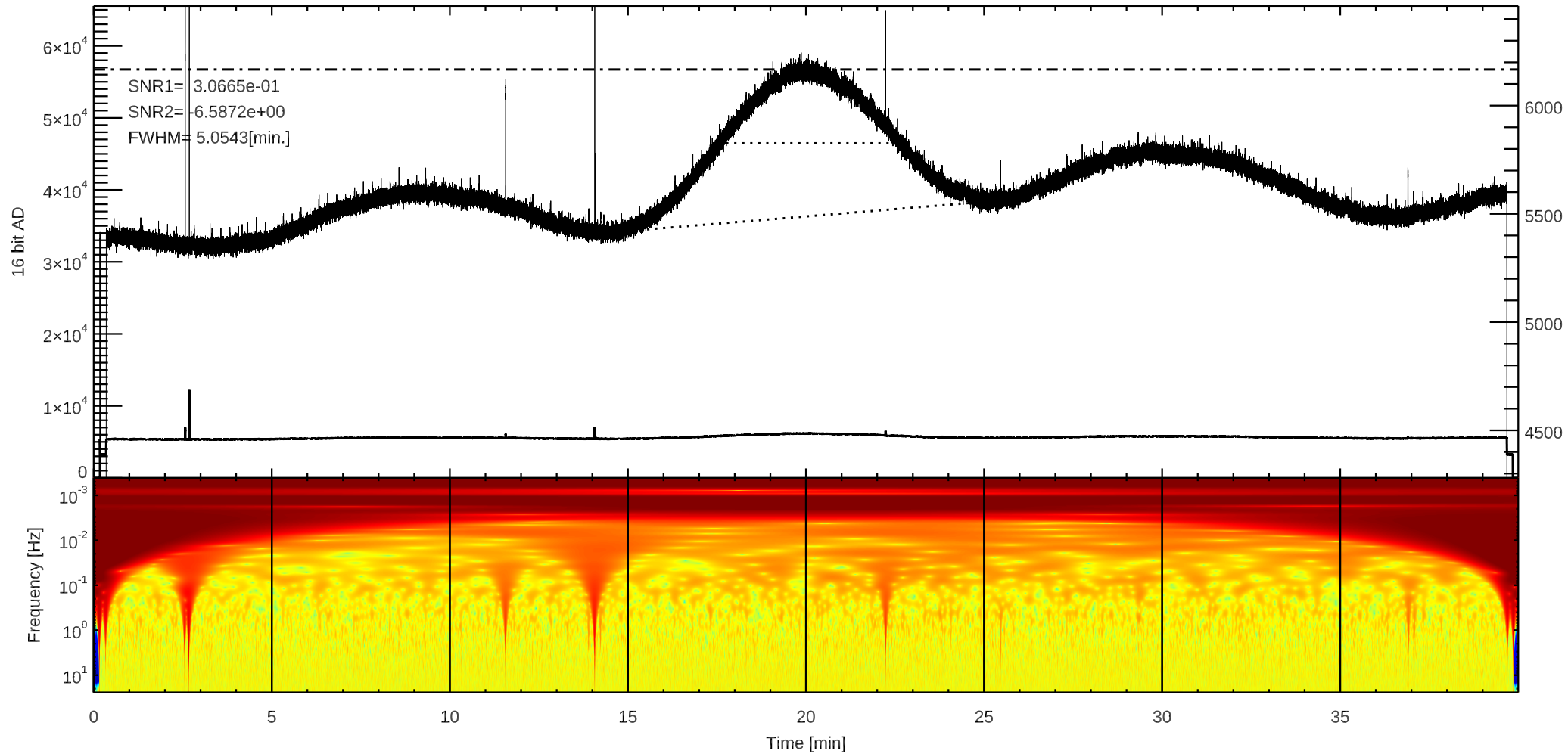
C 3C123 (/home4/archive/swift/dat/2023/10/T20231031013408.dat)
