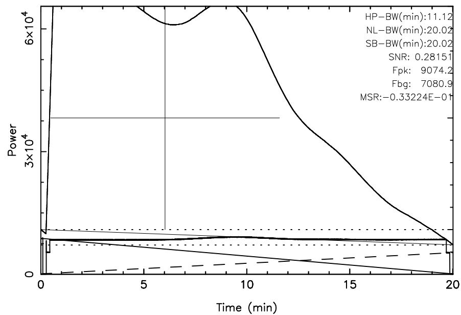
KISO 3C157 2023/10/03(276)05:14:47-05:34:48JST
