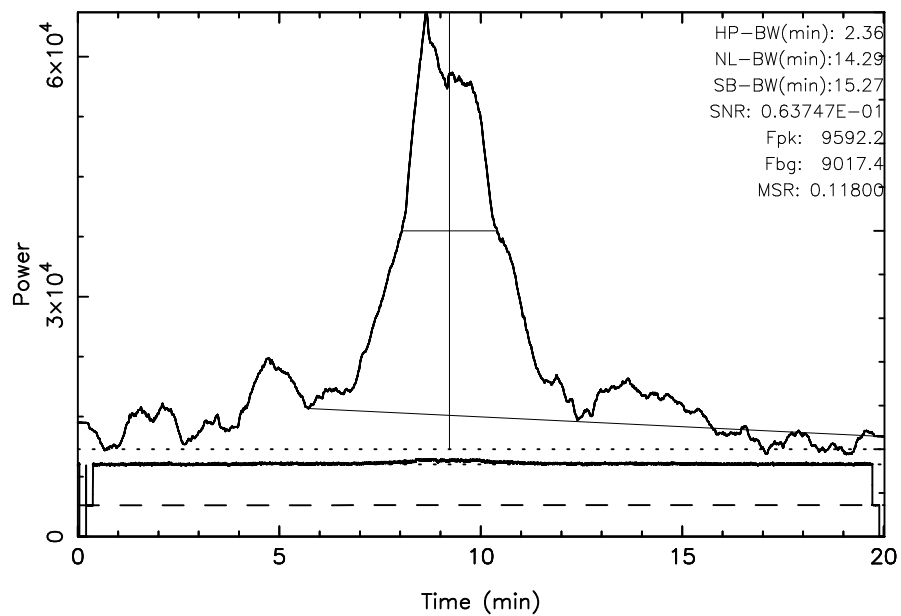
FUJI 3C157 2023/10/03(276)05:14:47-05:34:48JST
