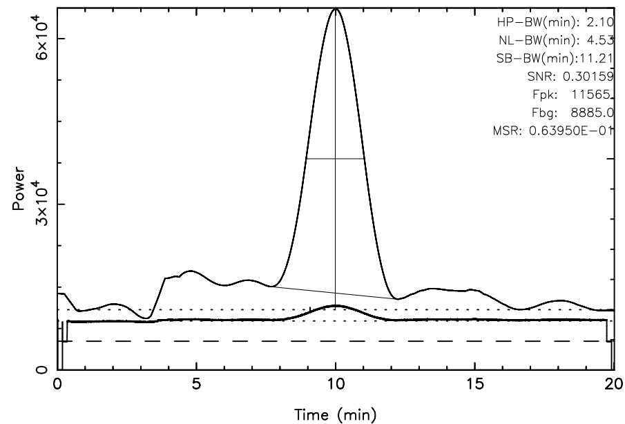
FUJI 3C144 2023/10/06(279)04:19:35-04:39:36JST
