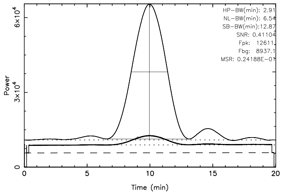
KISO 3C144 2023/10/06(279)04:19:35-04:39:36JST
