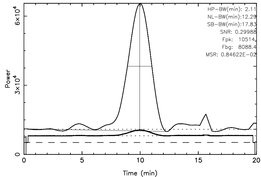
FUJI 3C144 2023/10/09(282)04:07:48-04:27:49JST
