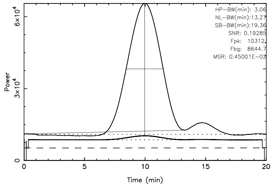
KISO 3C144 2023/10/09(282)04:07:48-04:27:49JST
