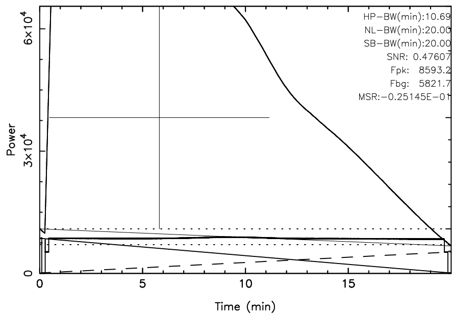
KISO 3C157 2023/10/09(282)04:51:13-05:11:13JST
