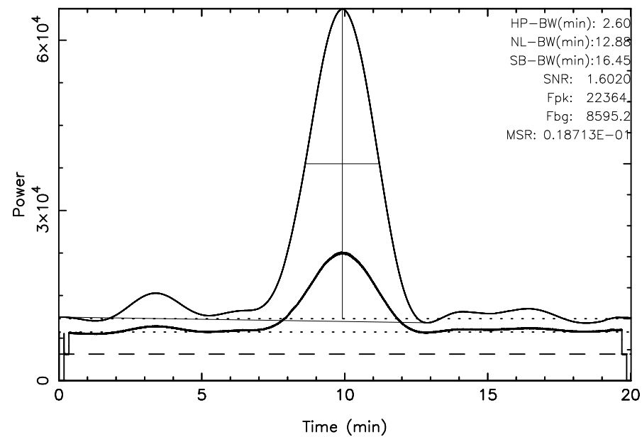
FUJI 3C405 2023/10/09(282)18:29:47-18:49:48JST
