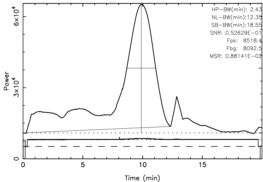
FUJI 3C123 2023/10/09(282)03:10:36-03:30:35JST
