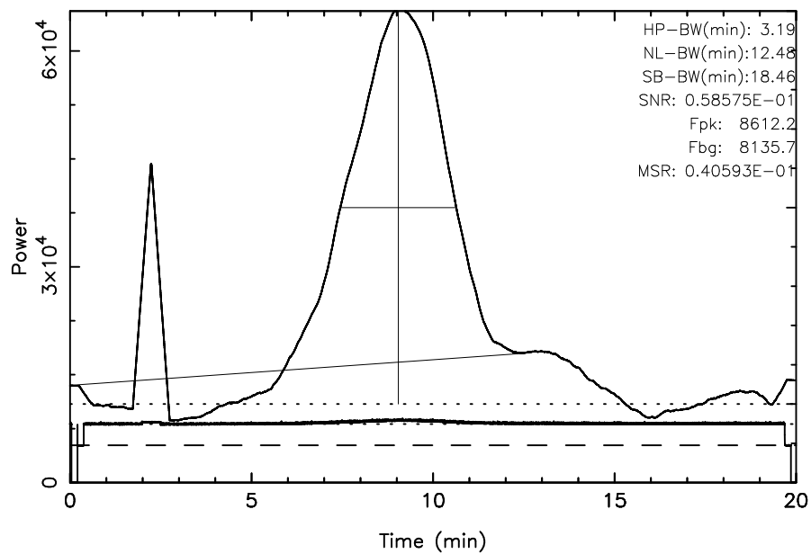
FUJI 3C157 2023/10/09(282)04:51:13-05:11:13JST
