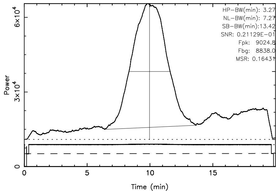
KISO 3C123 2023/10/09(282)03:10:36-03:30:35JST
