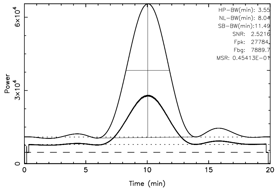
KISO 3C405 2023/10/09(282)18:29:47-18:49:48JST
