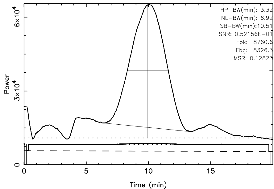
KISO 3C123 2023/10/11(284)03:02:44-03:22:44JST
