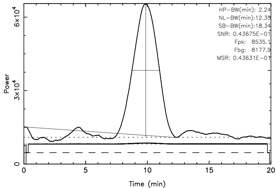
FUJI 3C123 2023/10/11(284)03:02:44-03:22:44JST
