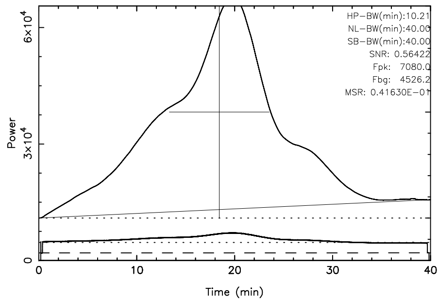
TOYOKAWA 3C392 2023/09/30(273)17:52:22-18:32:22JST
