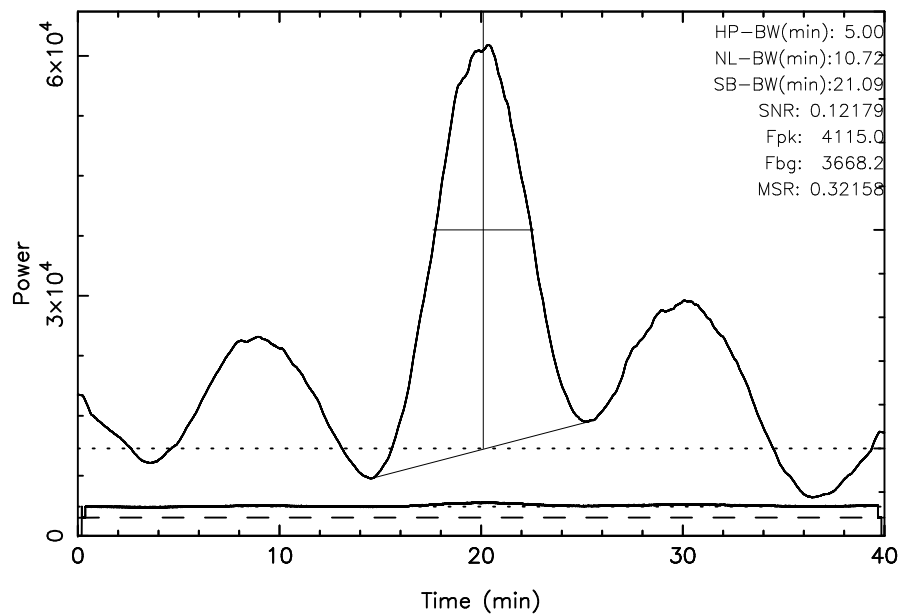
TOYOKAWA 3C123 2023/09/30(273)03:35:59-04:15:59JST
