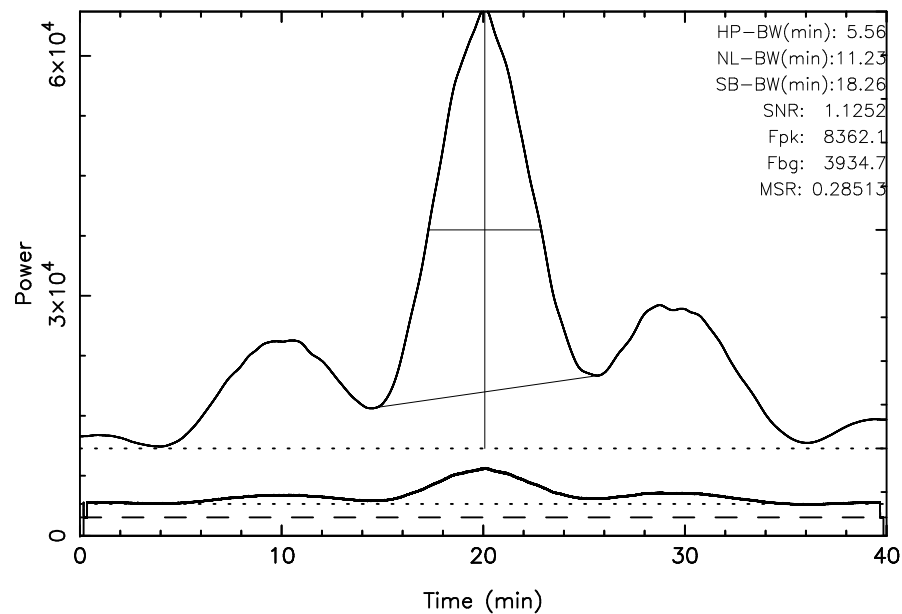
TOYOKAWA 3C144 2023/09/30(273)04:33:12-05:13:12JST
