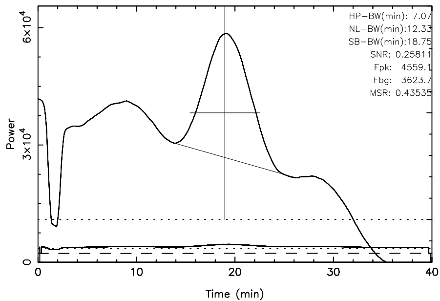
TOYOKAWA 3C157 2023/09/30(273)05:16:36-05:56:36JST
