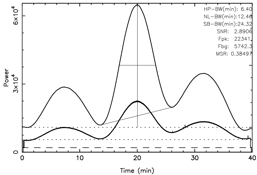
TOYOKAWA 3C405 2023/09/30(273)18:55:11-19:35:11JST
