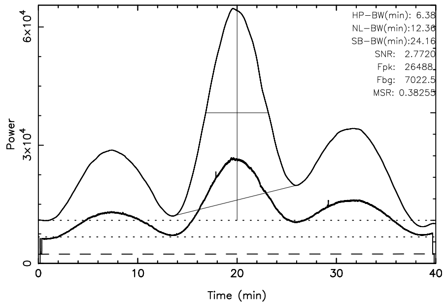
TOYOKAWA 3C405 2023/10/02(275)18:47:19-19:27:19JST
