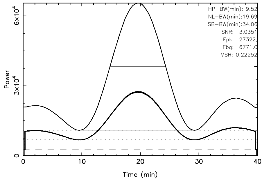
TOYOKAWA 3C461 2023/10/03(276)22:06:59-22:46:59JST
