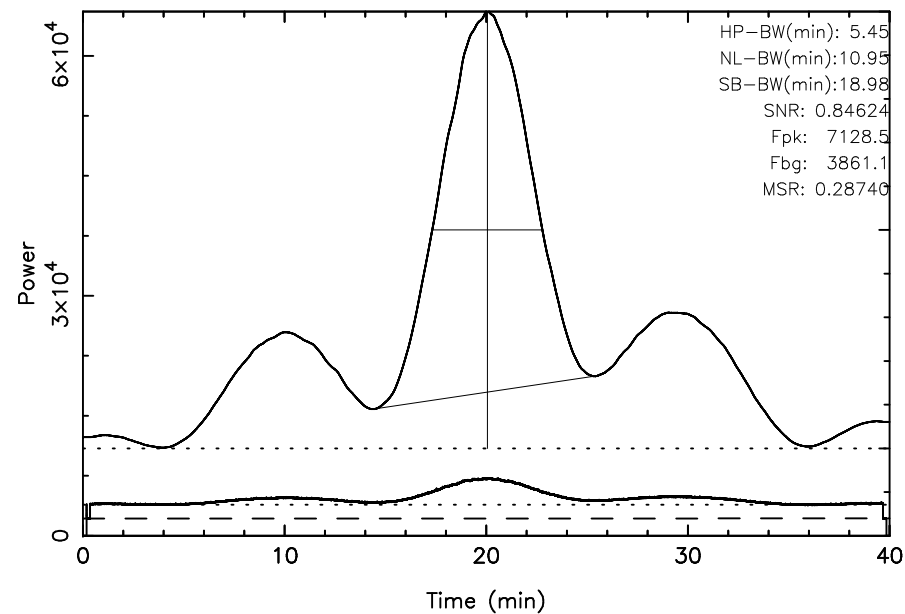
TOYOKAWA 3C144 2023/10/03(276)04:21:24-05:01:24JST
