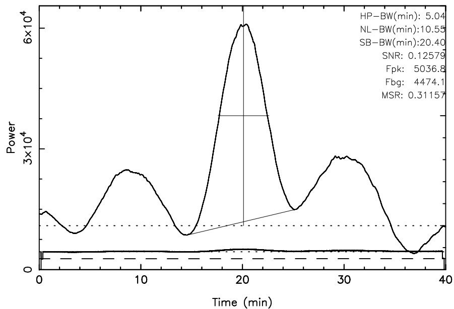
TOYOKAWA 3C123 2023/10/03(276)03:24:11-04:04:11JST
