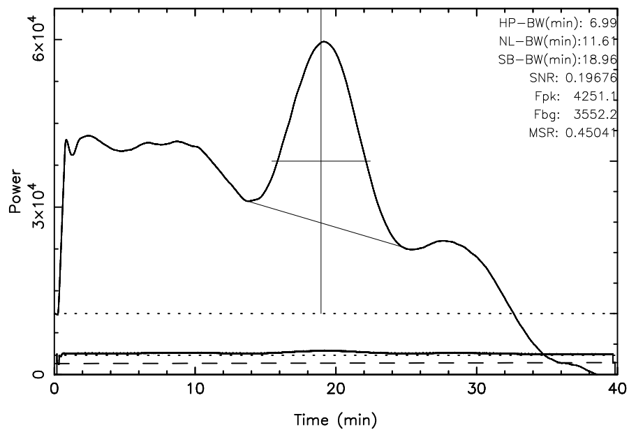
TOYOKAWA 3C157 2023/10/03(276)05:04:48-05:44:48JST
