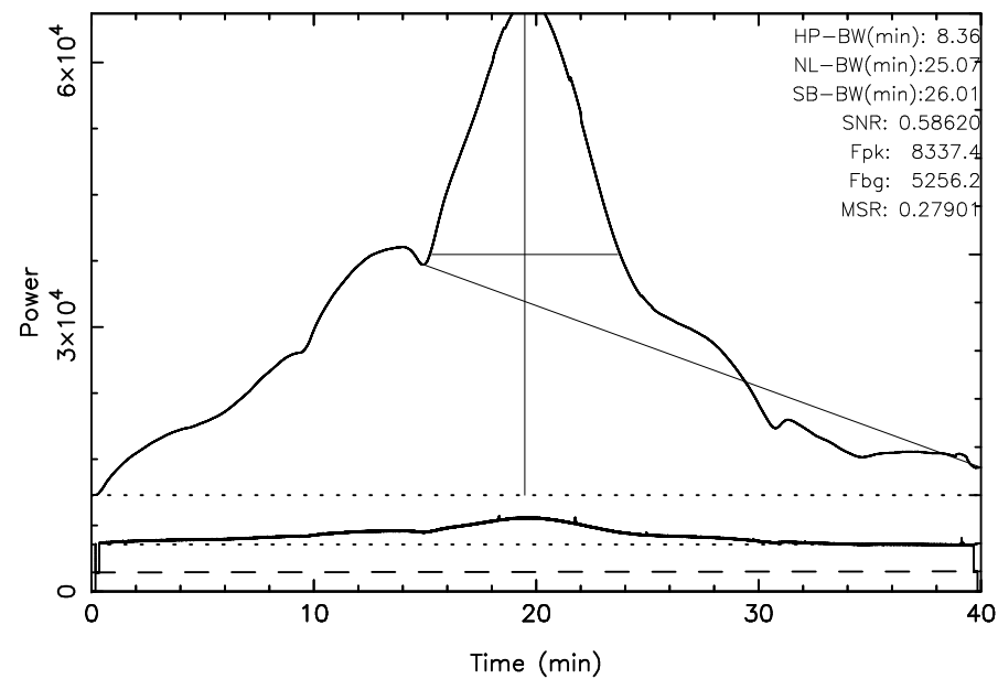
TOYOKAWA 3C392 2023/10/03(276)17:40:34-18:20:34JST
