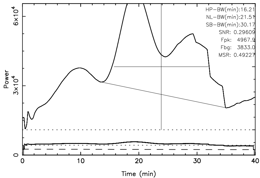
TOYOKAWA 3C157 2023/10/09(282)04:41:13-05:21:13JST
