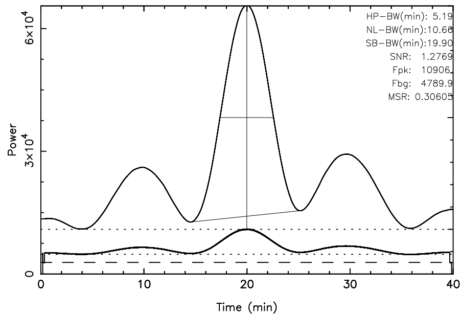
TOYOKAWA 3C144 2023/10/09(282)03:57:49-04:37:49JST
