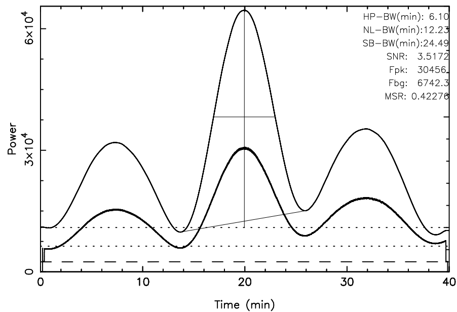
TOYOKAWA 3C405 2023/10/09(282)18:19:48-18:59:48JST
