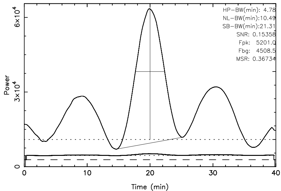
TOYOKAWA 3C123 2023/10/09(282)03:00:36-03:40:36JST
