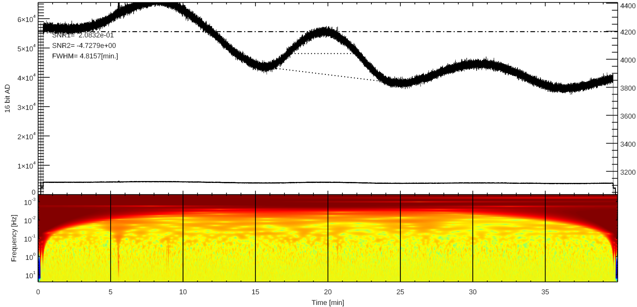
C 3C123 (/home4/archive/swift/dat/2023/11/T20231101013012.dat)
