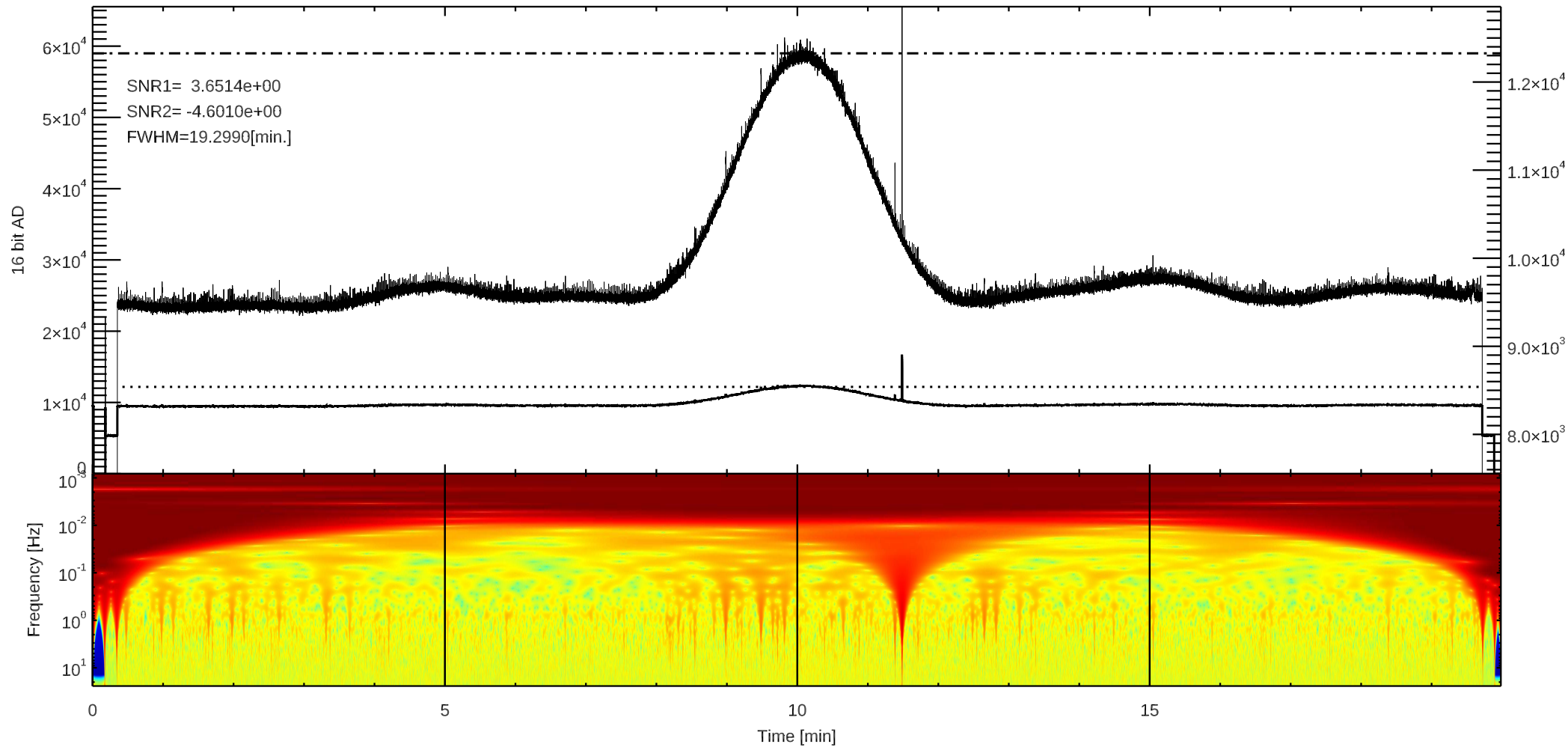
C 3C144 (/home4/archive/fit/dat/2023/11/F20231103022933.dat)
