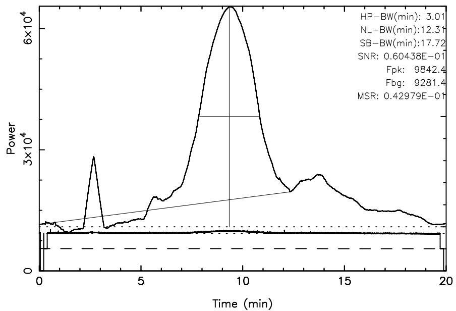
FUJI 3C157 2023/11/01(305)03:20:47-03:40:47JST
