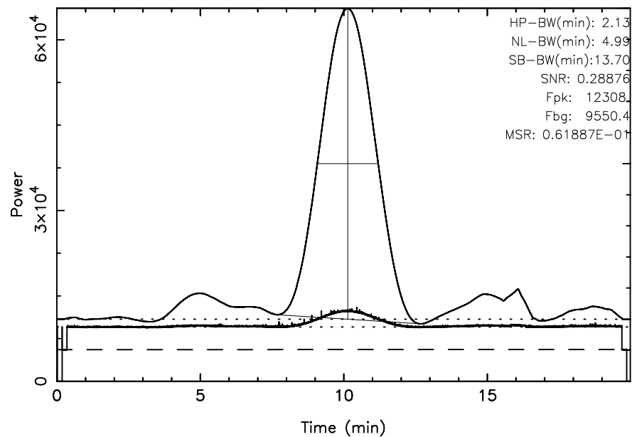
FUJI 3C144 2023/11/01(305)02:37:23-02:57:22JST
