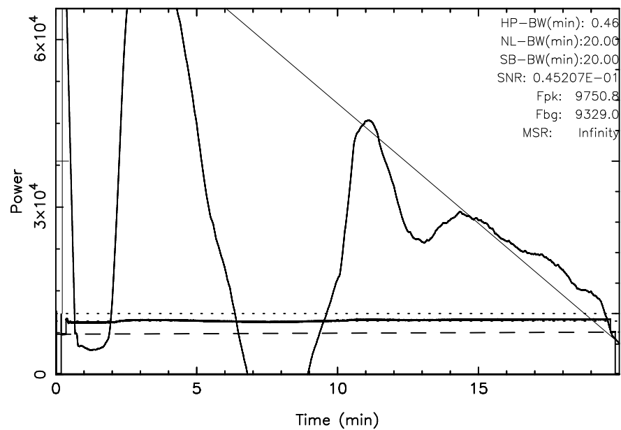
KISO 3C123 2023/11/01(305)01:40:09-02:00:09JST
