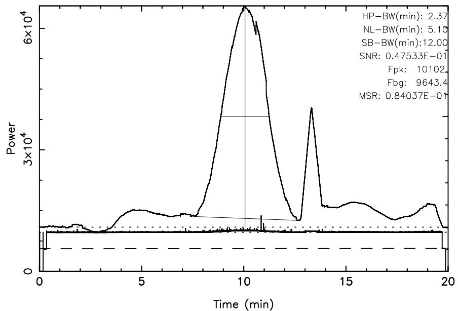
FUJI 3C123 2023/11/01(305)01:40:09-02:00:09JST
