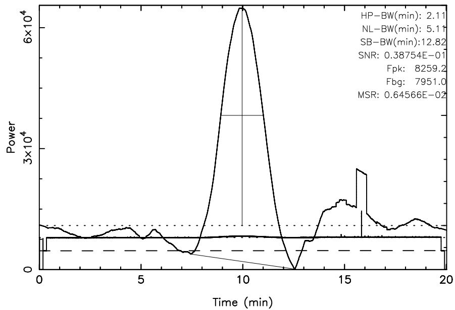
FUJI 3C123 2023/11/11(315)01:00:50-01:20:51JST
