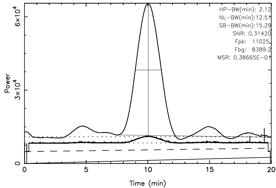
FUJI 3C144 2023/11/11(315)01:58:03-02:18:03JST
