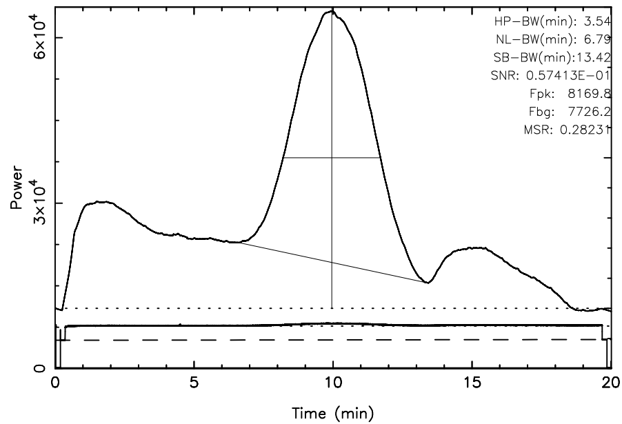
KISO 3C123 2023/11/11(315)01:00:50-01:20:51JST
