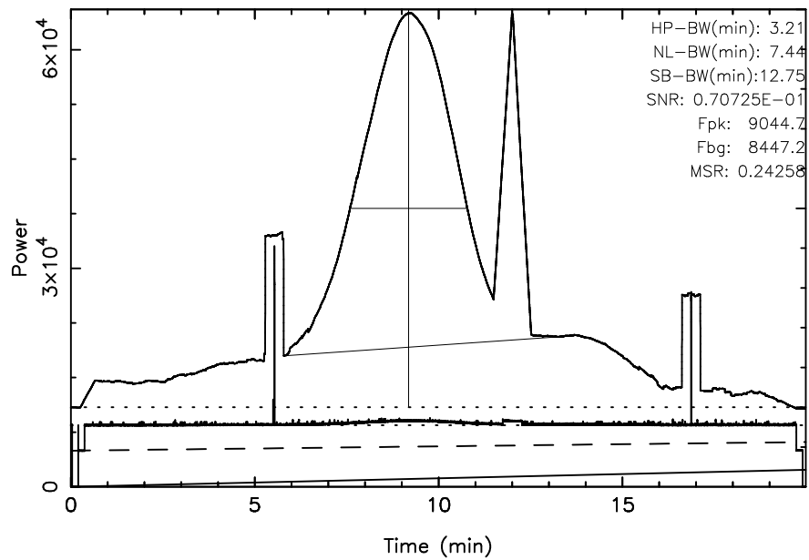
FUJI 3C157 2023/11/11(315)02:41:28-03:01:27JST
