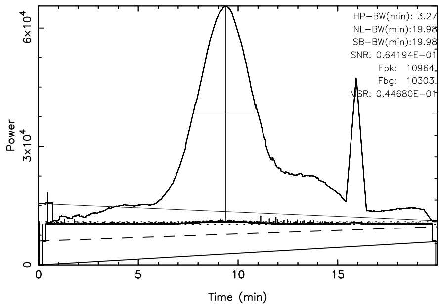
FUJI 3C157 2023/11/12(316)02:37:32-02:57:31JST
