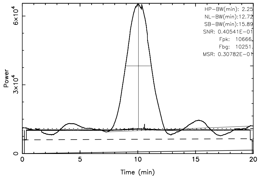
FUJI 3C123 2023/11/12(316)00:56:55-01:16:55JST
