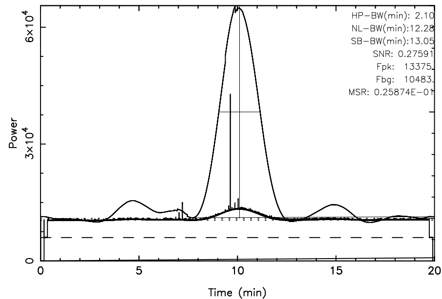
FUJI 3C144 2023/11/12(316)01:54:07-02:14:07JST
