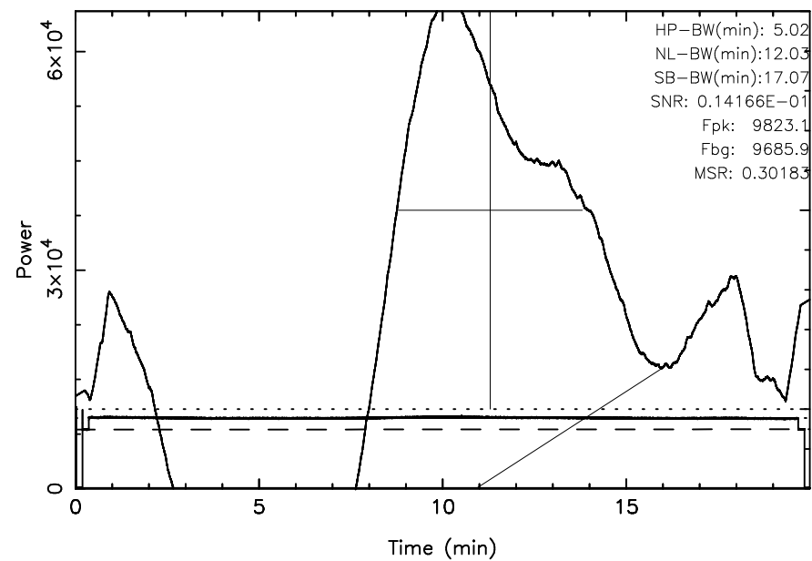
KISO 3C123 2023/11/12(316)00:56:55-01:16:55JST
