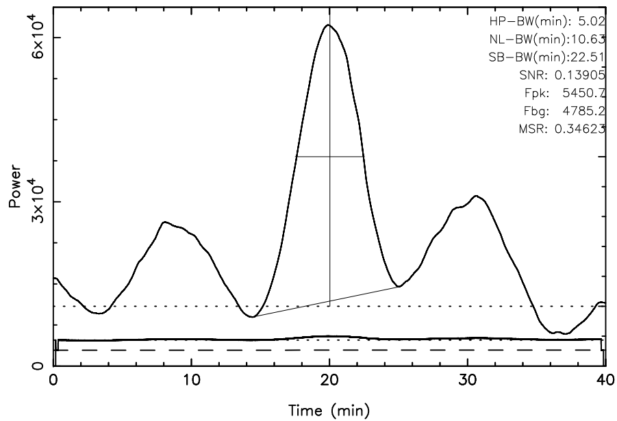
TOYOKAWA 3C123 2023/11/05(309)01:14:27-01:54:27JST
