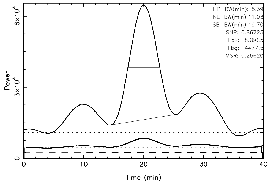
TOYOKAWA 3C144 2023/11/05(309)02:11:39-02:51:39JST
