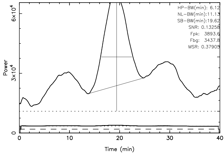
TOYOKAWA 3C157 2023/11/05(309)02:55:04-03:35:04JST
