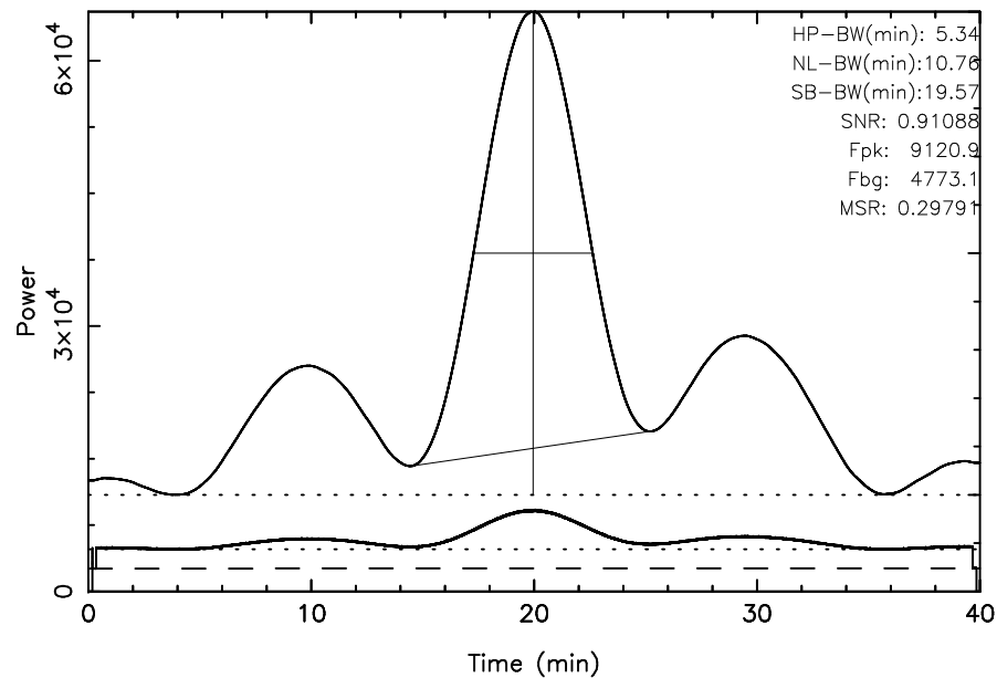
TOYOKAWA 3C144 2023/11/13(317)01:40:12-02:20:12JST
