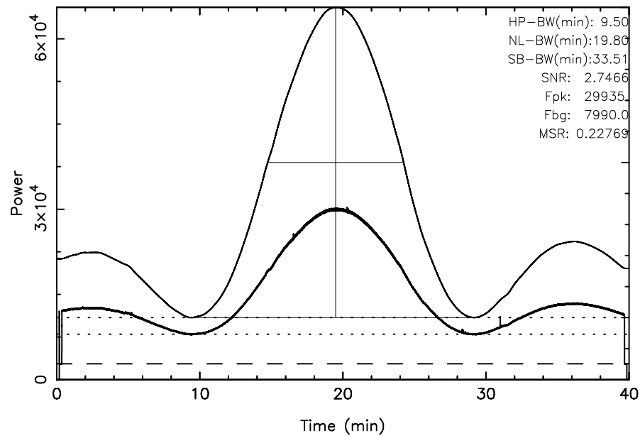
TOYOKAWA 3C461 2023/11/13(317)19:25:47-20:05:47JST
