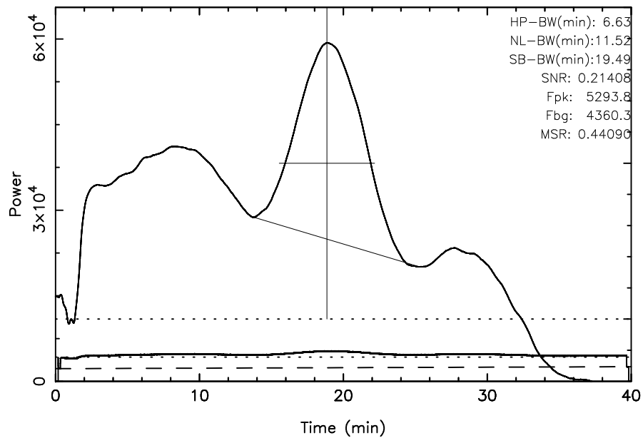
TOYOKAWA 3C157 2023/11/13(317)02:23:36-03:03:36JST
