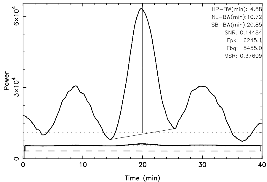
TOYOKAWA 3C123 2023/11/13(317)00:42:59-01:22:59JST
