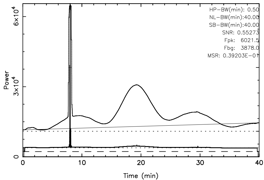
TOYOKAWA 3C157 2023/11/17(321)02:07:53-02:47:53JST
