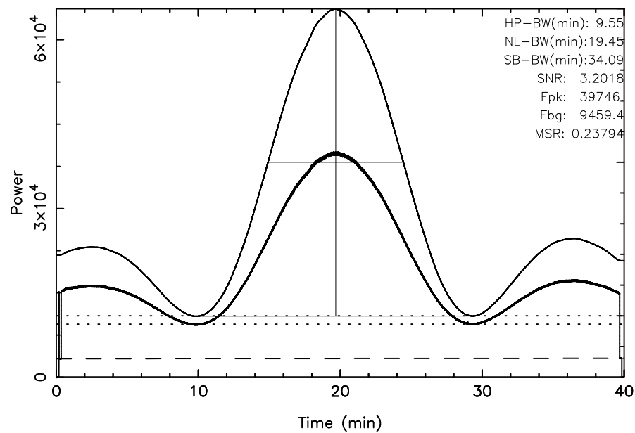
TOYOKAWA 3C461 2023/11/17(321)19:10:04-19:50:04JST
