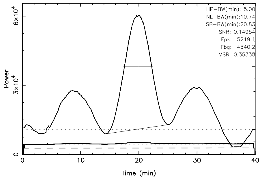
TOYOKAWA 3C123 2023/11/17(321)00:27:16-01:07:16JST
