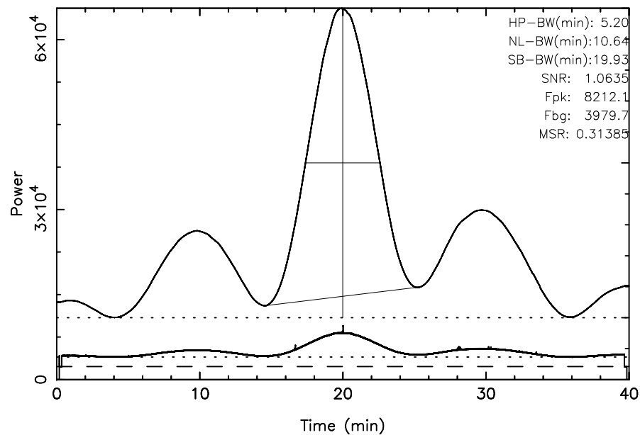
TOYOKAWA 3C144 2023/11/17(321)01:24:29-02:04:29JST
