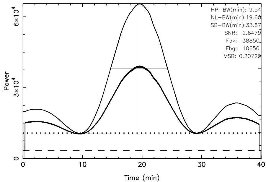
TOYOKAWA 3C461 2023/11/23(327)18:46:28-19:26:28JST
