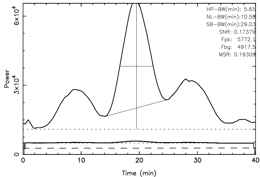
TOYOKAWA 3C157 2023/11/23(327)01:44:17-02:24:17JST
