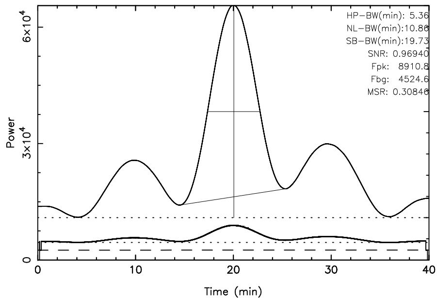
TOYOKAWA 3C144 2023/11/24(328)00:56:57-01:36:57JST
