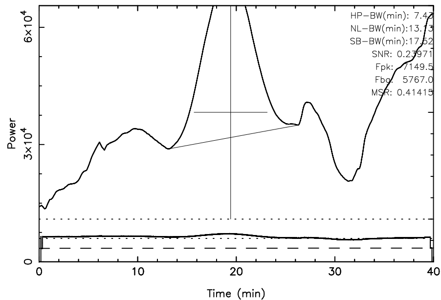
TOYOKAWA 3C157 2023/11/27(331)01:28:34-02:08:34JST
