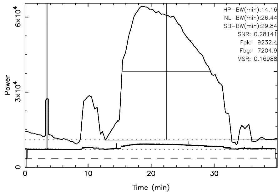
TOYOKAWA 3C10 2023/12/04(338)19:05:21-19:45:21JST
