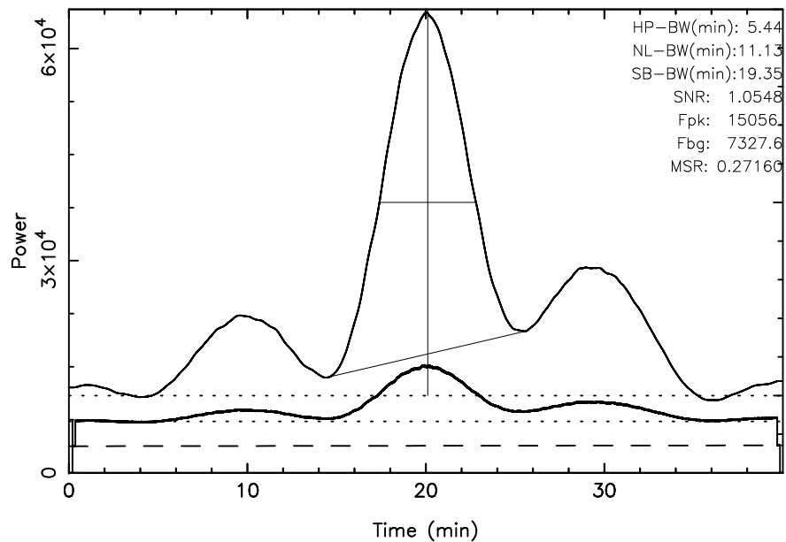
TOYOKAWA 3C144 2023/12/04(338)00:17:38-00:57:38JST
