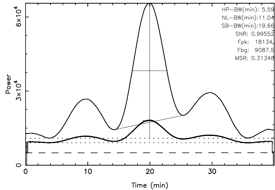
TOYOKAWA 3C144 2023/12/26(360)22:47:13-23:27:13JST
