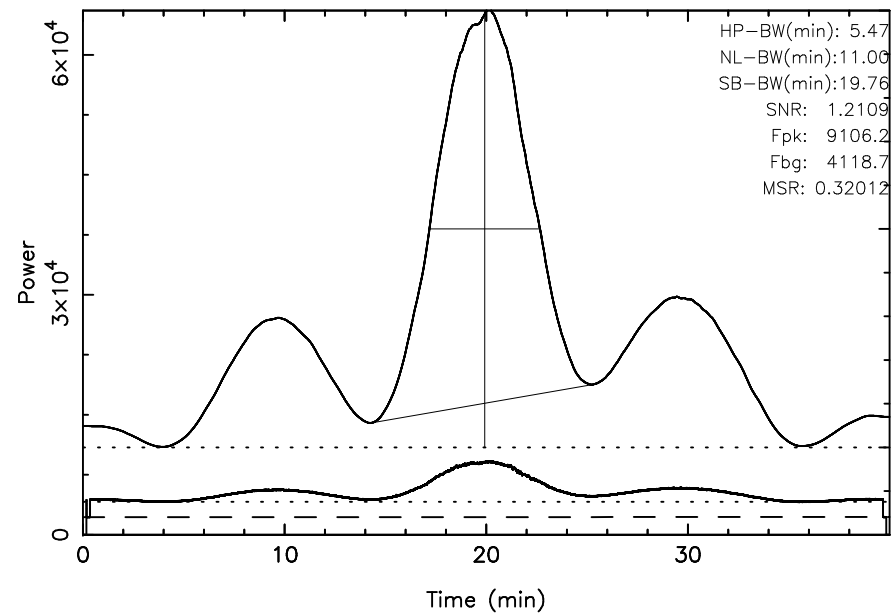
TOYOKAWA 3C144 2024/01/02(002)22:19:41-22:59:41JST
