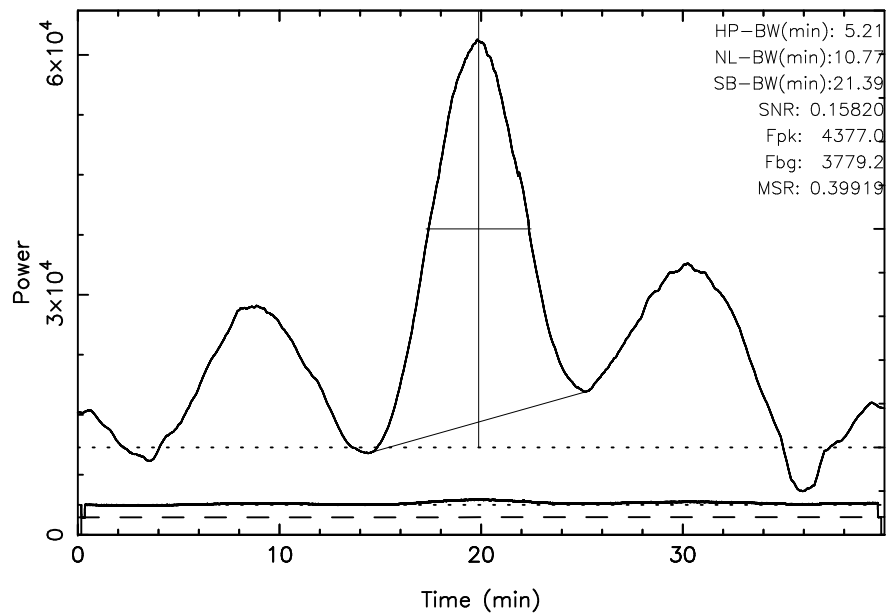
TOYOKAWA 3C123 2024/01/02(002)21:22:28-22:02:28JST
