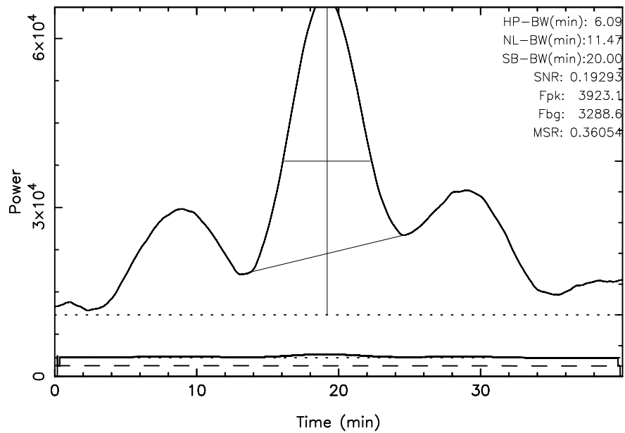
TOYOKAWA 3C157 2024/01/02(002)23:03:06-23:43:06JST
