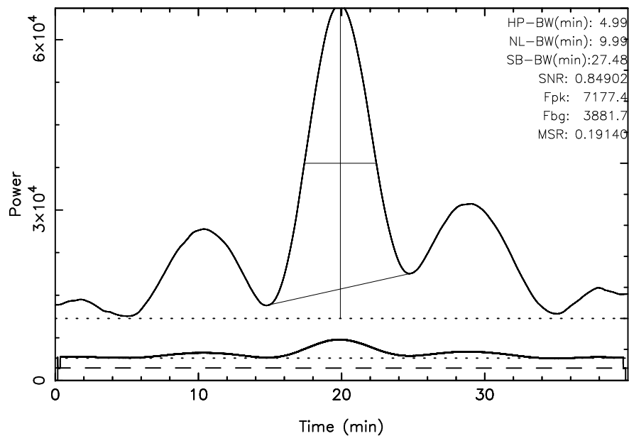
TOYOKAWA 3C274 2024/01/08(008)04:54:58-05:34:58JST
