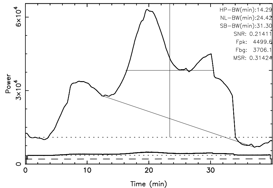
TOYOKAWA 3C123 2024/01/08(008)20:58:53-21:38:53JST
