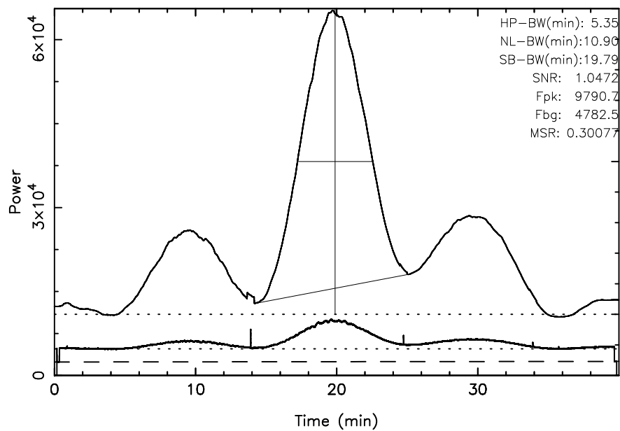
TOYOKAWA 3C144 2024/01/08(008)21:56:06-22:36:06JST
