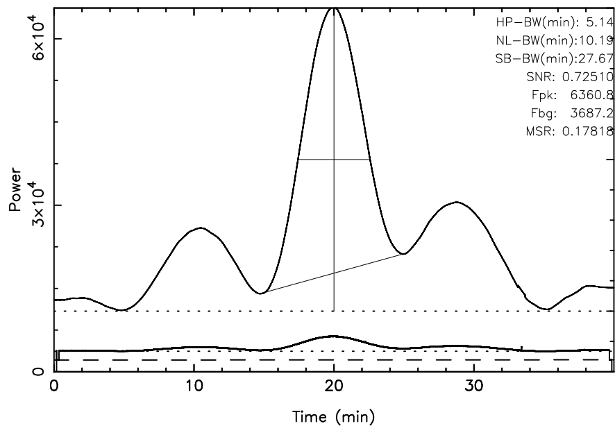
TOYOKAWA 3C274 2024/01/10(010)04:47:06-05:27:06JST
