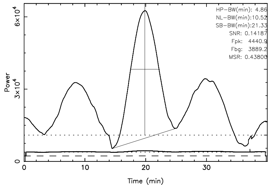
TOYOKAWA 3C123 2024/01/10(010)20:51:01-21:31:01JST
