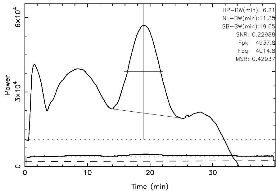
TOYOKAWA 3C157 2024/01/10(010)22:31:38-23:11:38JST
