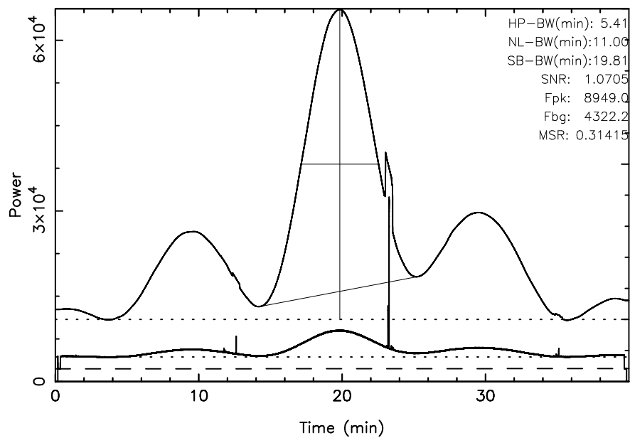
TOYOKAWA 3C144 2024/01/10(010)21:48:14-22:28:14JST
