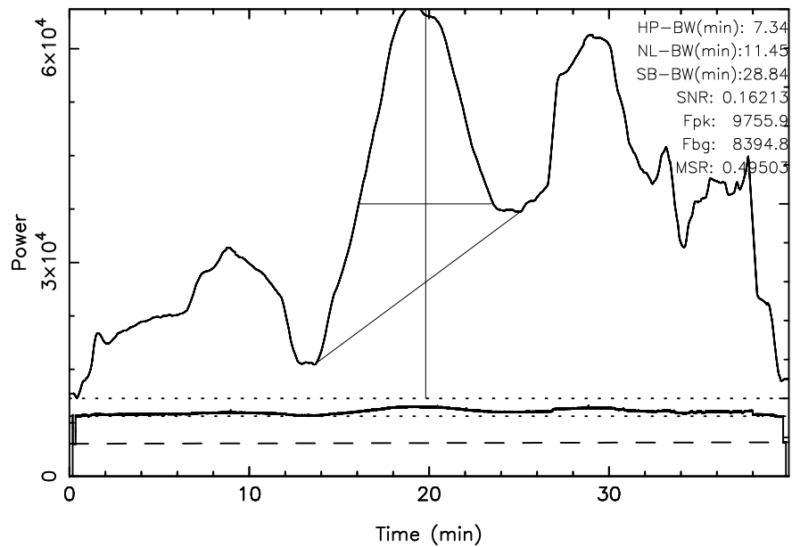
TOYOKAWA 3C157 2024/01/11(011)22:27:42-23:07:42JST
