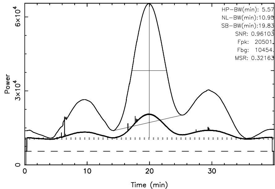
TOYOKAWA 3C144 2024/01/11(011)21:44:18-22:24:18JST
