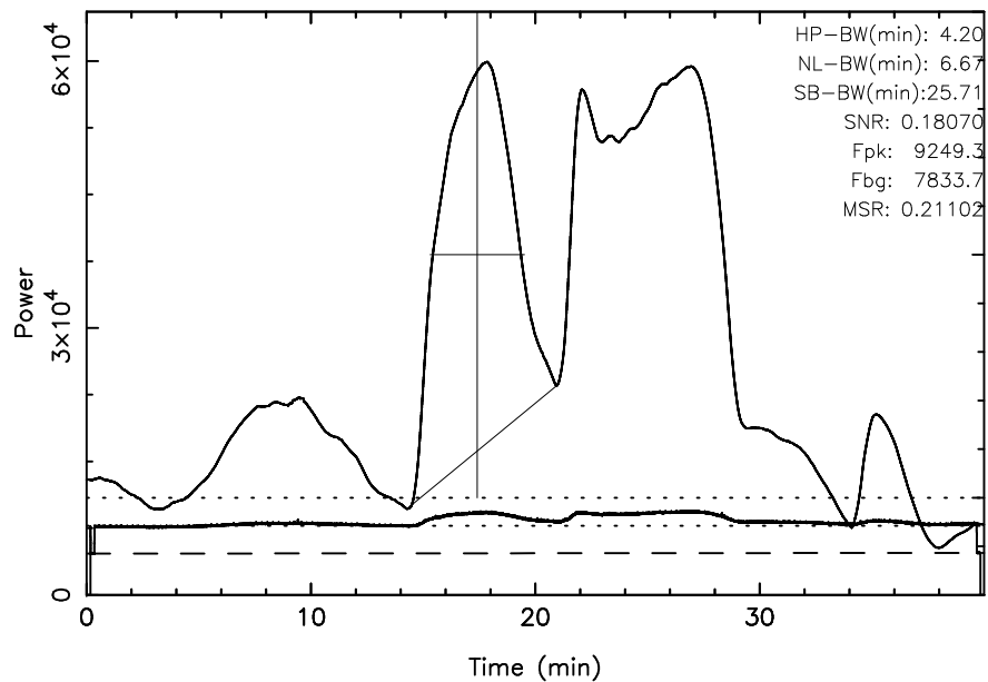
TOYOKAWA 3C123 2024/01/11(011)20:47:05-21:27:05JST
