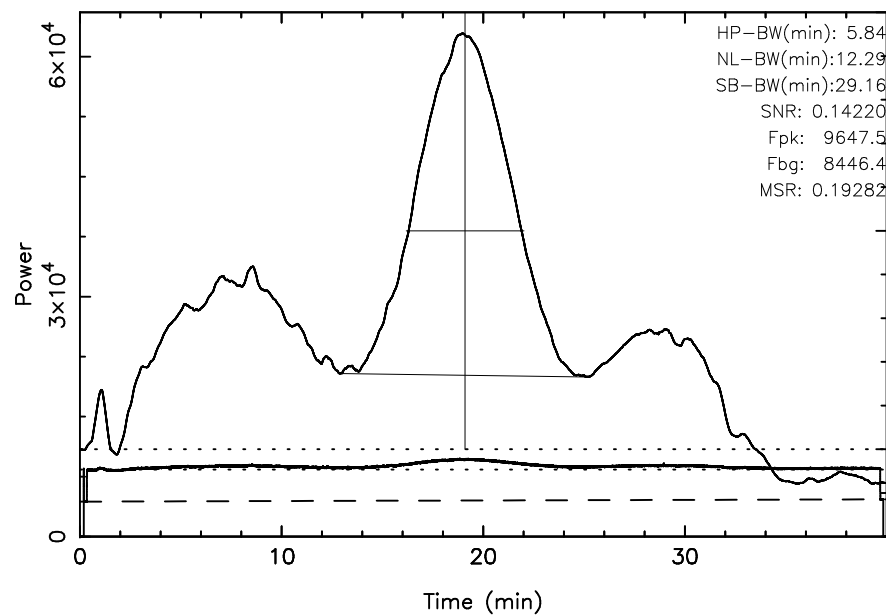
TOYOKAWA 3C157 2024/01/13(013)22:19:51-22:59:51JST
