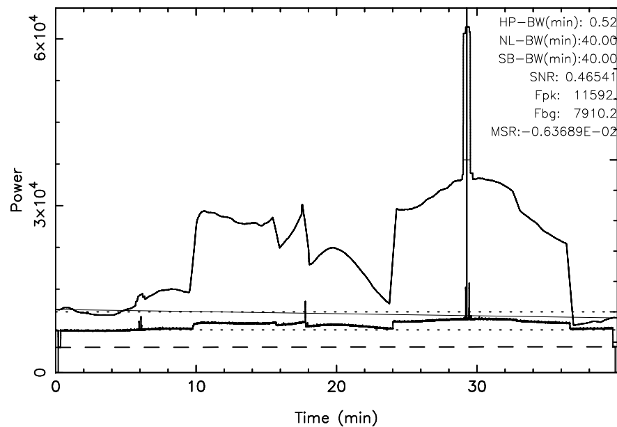
TOYOKAWA 3C123 2024/01/13(013)20:39:14-21:19:14JST
