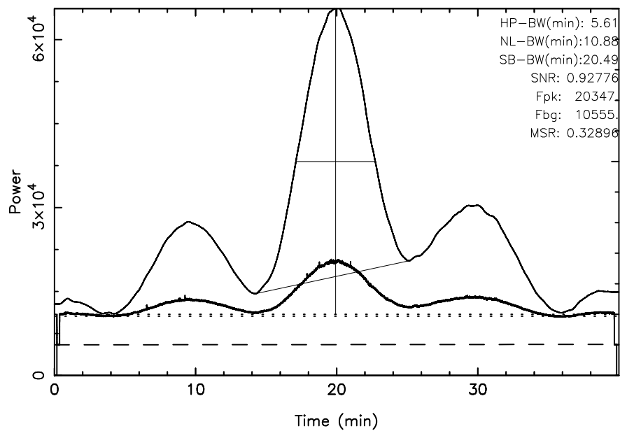
TOYOKAWA 3C144 2024/01/13(013)21:36:26-22:16:26JST
