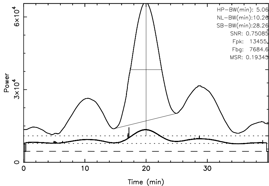
TOYOKAWA 3C274 2024/01/13(013)04:35:18-05:15:18JST
